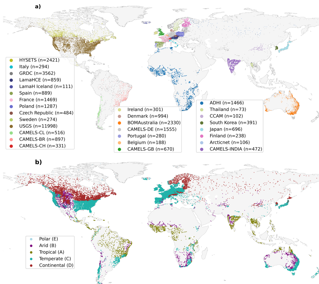
Figure 1. Locations of the 35 254 gauges with daily streamflow data that passed the duplication checks, used to evaluate the gridded P datasets. Each data point represents the centroid of a catchment. The colors indicate the dominant major Köppen-Geiger climate class, based on the 1 km resolution map for 1991–2020 from Beck et al. (2023). For more information on the streamflow data sources, refer to Appendix A.
