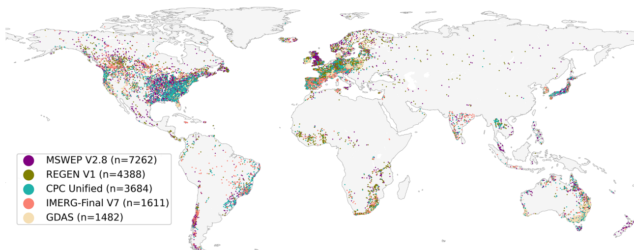
Figure 3. Precipitation ( P ) dataset with the highest calibration KGE in each catchment. Points mark catchment centroids ( n = 18\,428 ). For clarity, only the five datasets with the highest median KGE are shown. MSWEP-np V2.8 is omitted because it is highly similar to MSWEP V2.8.
