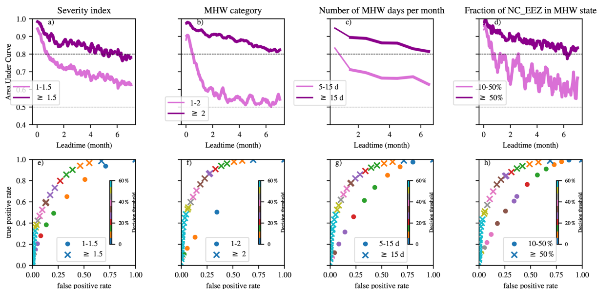
Figure 7. Probabilistic forecast skill of the ECMWF system SEAS5 (cf legend of Fig. 6).
