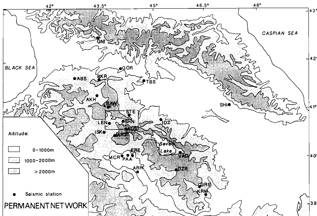
Figure 7. Topographical map of Caucasus with the sites of regional (Armenian, Georgian and Azerbaijanian) stations used for relocations. The rectangle shows the region surveyed by the portable network after the Spitak earthquake.
