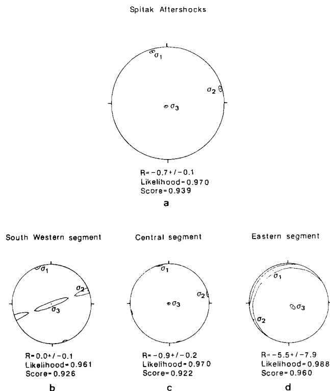
Figure 5. Principal axes of the stress tensors in lower hemisphere Schmidt equal area projection. One standard deviation ellipses around the axes are shown. The shape factor R = (\sigma_z - \sigma_x)/(\sigma_y - \sigma_x) indicates the stress regime (Rivera & Cisternas 1990). (a) Total data set of the aftershocks of Table 2. (b) South western segment. (c) Spitak-Gekhasar central segment. (d) Alavar eastern segment. Negative values of R correspond to triaxial compression, but the tensor has symmetries in cases (b), where two different faults are mixed, and (d) where we have almost one single fault plane.
