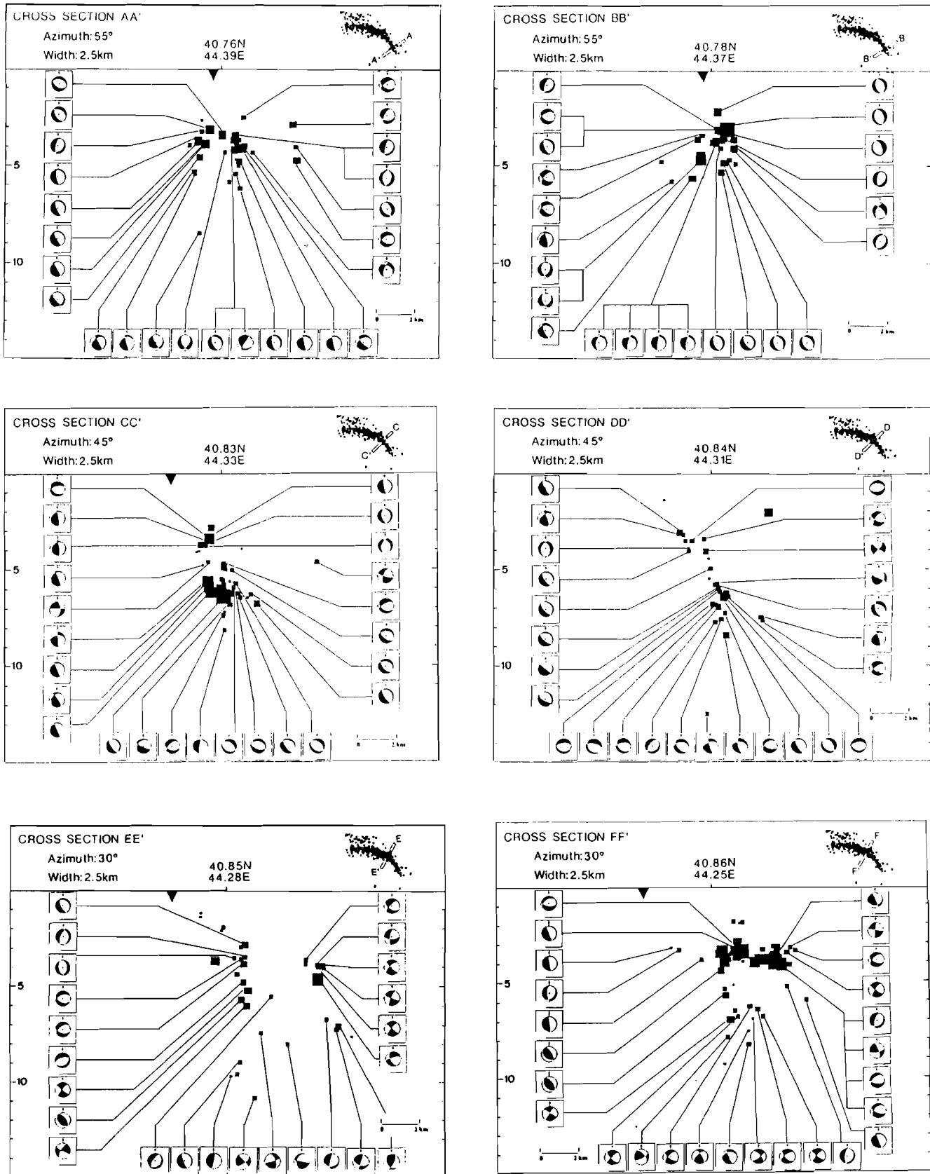
Figure 4. Cross-sections (AA' to FF') through the hypocentres of the aftershocks along the lines shown in the insets. No vertical exaggeration. Depth estimations have 1400 m above sea-level as reference level. The focal mechanisms are shown in the Schmidt equal area back projection roughly looking NW. An inverted triangle at the surface shows the trace of the fault, while the filled half circle indicates the position of an anticline. The coordinates of the central point of the section, its width and its azimuth are shown.
