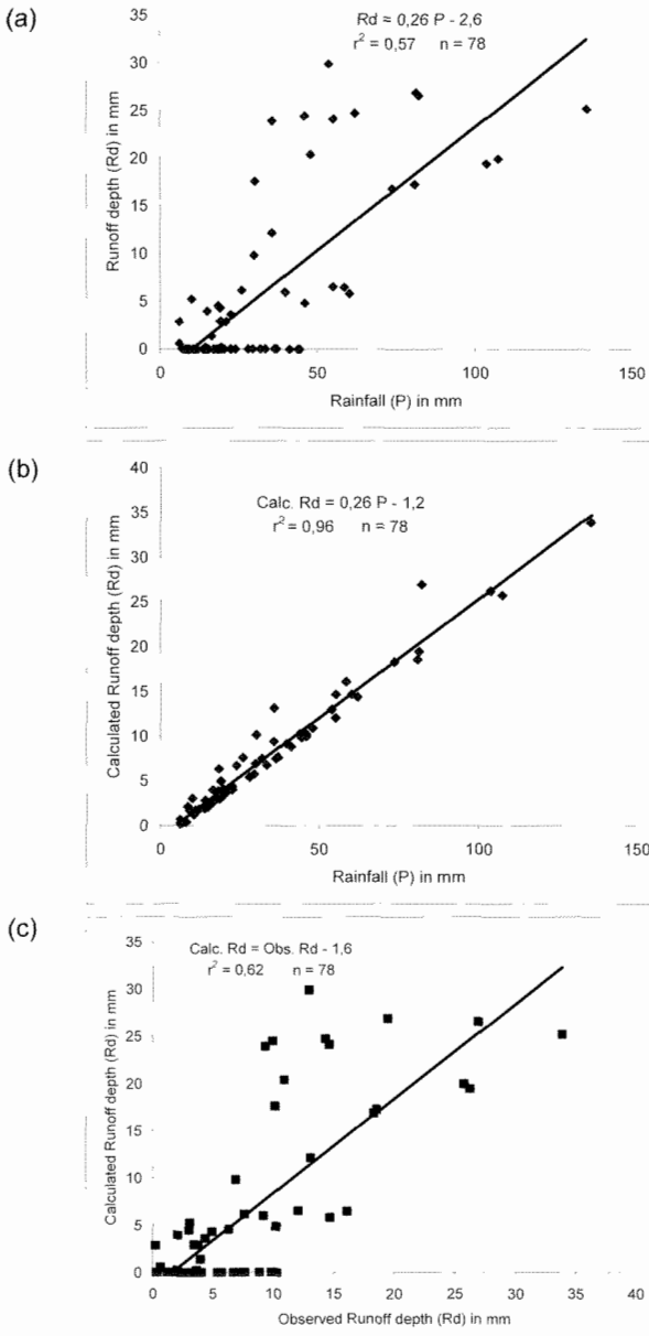
Fig. 4 Rainfall–runoff relationship (a) observed and (b) calculated by the Nazas model, for plot no. 4 (black marls, Orpierre site); and (c) the relationship between calculated and observed runoff depth for the same plot.
