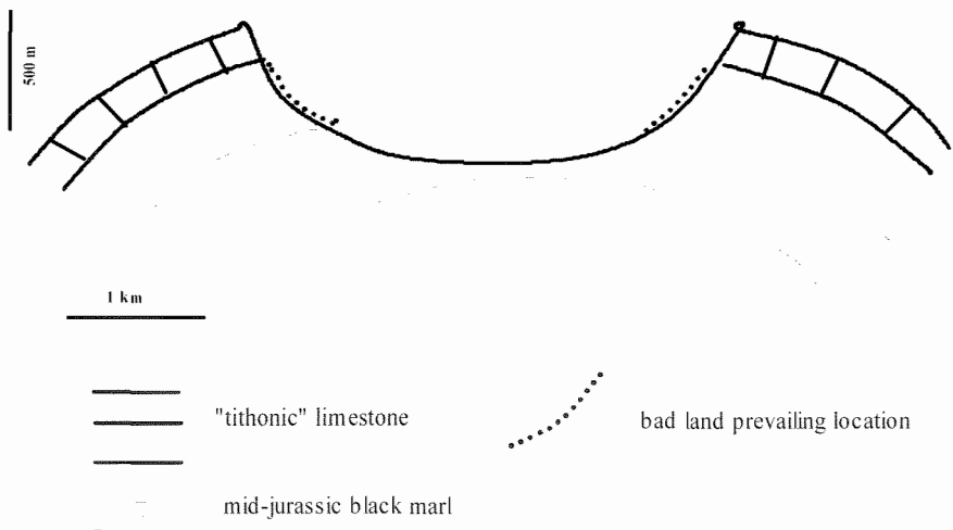
Fig. 3 The prevailing location of badlands on a cross section of a typical valley of the “Vocontian Graben” badlands are mostly located where the slope gradient and the intensity of overland flow are high. This explains why the dip–hillslope angle is commonly between 60 and 90%.
