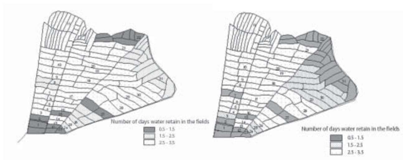
FIGURE 15. Number of days water is retained in the fields (two successive rotations).
