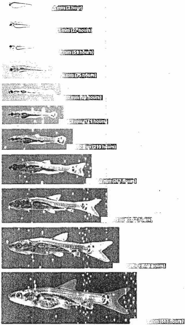
Plate 1. Illustration of the ontogeny of Balantiocheilos melanopterus
