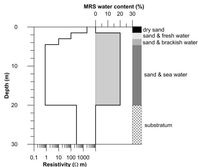
Fig. 1. Geoelectrical and water content models with a thickness of 1.5 m for the first 3 layers. Numerical modelling is conducted with a thickness of the first 3 layers ranging from 1.5 to 10 m and considering a water content of 20 % in medium- to coarse-grained sand ( T_2^* = 0.2 s).
