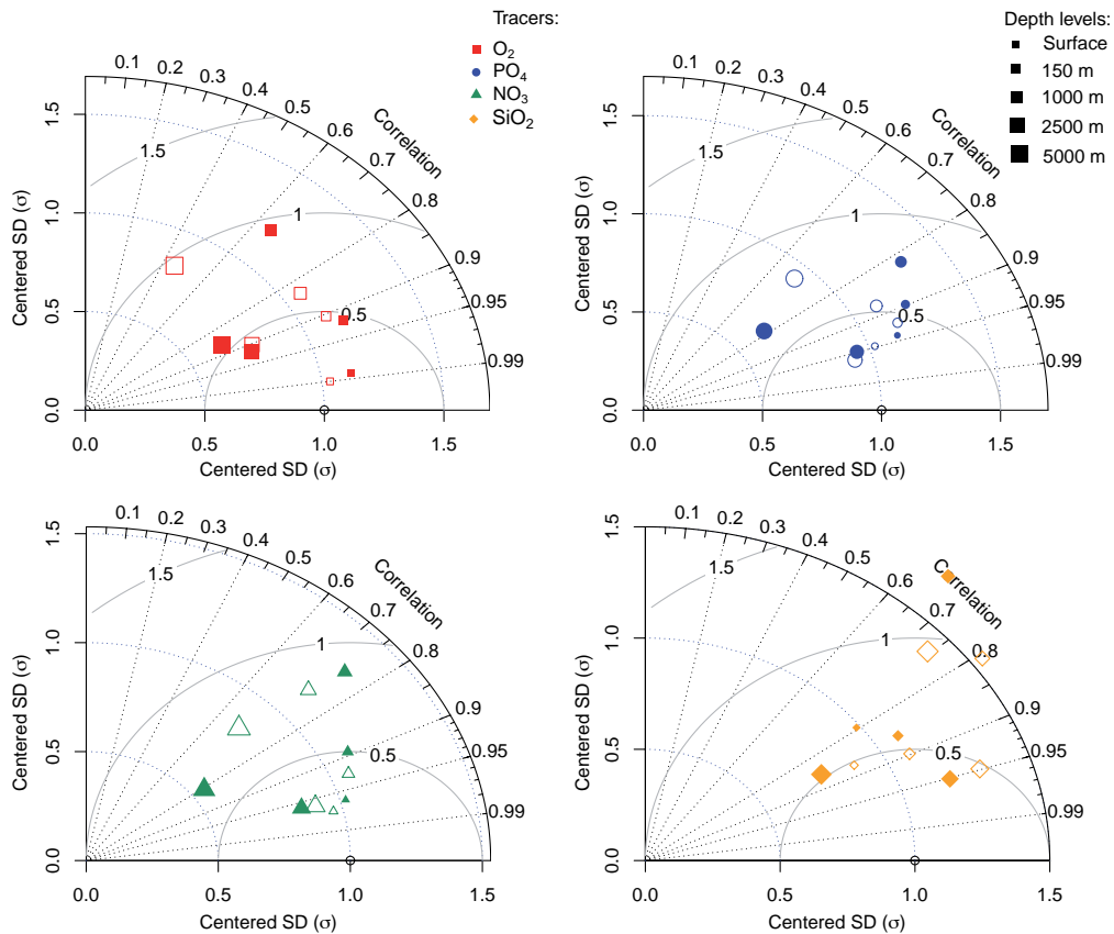
Figure 14. Taylor diagrams showing the correspondence between model results and observations for CNRM-ESM1 and CNRM-CM5.2 (S  ferian et al., 2013). Climatological distribution over 1986–2005 of simulated oxygen (O 2 ), phosphate (PO 4 ), nitrate (NO 3 ) and silicate (SiO 2 ) concentrations are assessed against WOA2013 data product. Filled and empty symbols indicate skills for CNRM-ESM1 and CNRM-CM5, respectively. The size of the symbols indicates the depth at which statistics have been computed.
