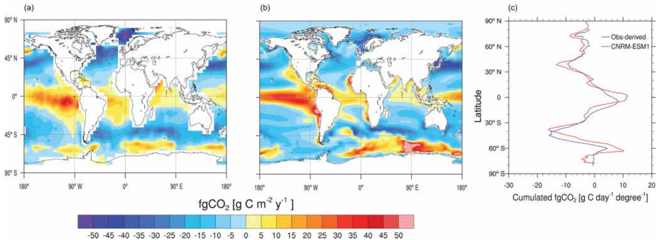
Figure 15. Annual-mean ocean carbon fluxes (fgCO 2 ) as estimated by the Takahashi et al. (2010) database (a) and as simulated by CNRM-ESM1 averaged over 1986–2005 (b). Panel (c) represents the zonal-cumulated carbon fluxes in function of latitude for both observation-based estimates (in blue) and CNRM-ESM1 (in red). Negative (positive) fluxes indicate an uptake (outgassing) of CO 2 .
