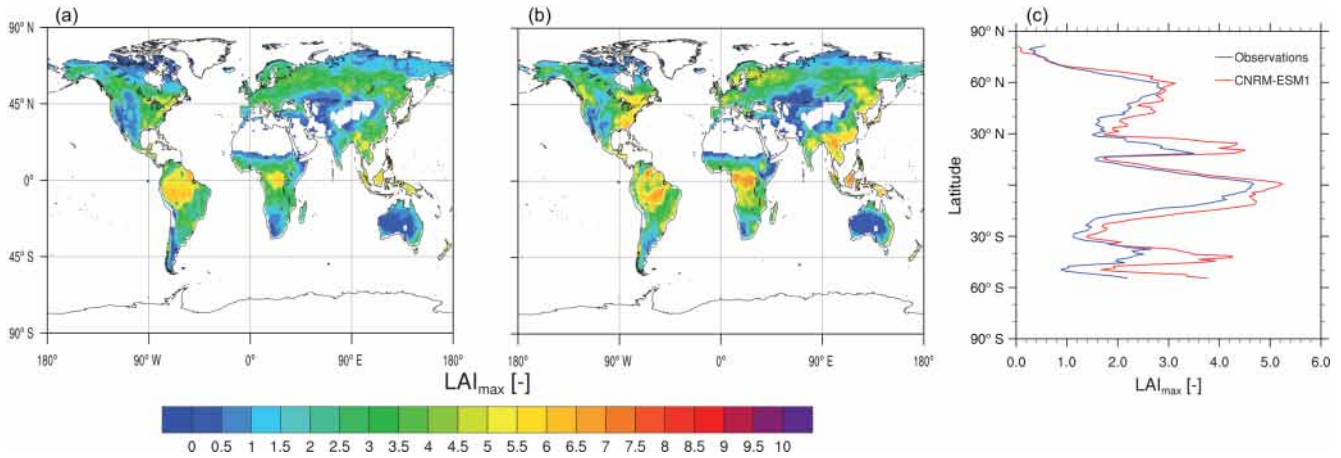
Figure 17. Composite of yearly maximum of leaf area index (LAI max ) as estimated from AVHRR satellite observations of Zhu et al. (2013) (a) and as simulated by CNRM-ESM1 (b) over 1986–2005. Panel (c) represents the zonal-average LAI max in function of latitude for both observation-based estimates (in blue) and CNRM-ESM1 (in red).
