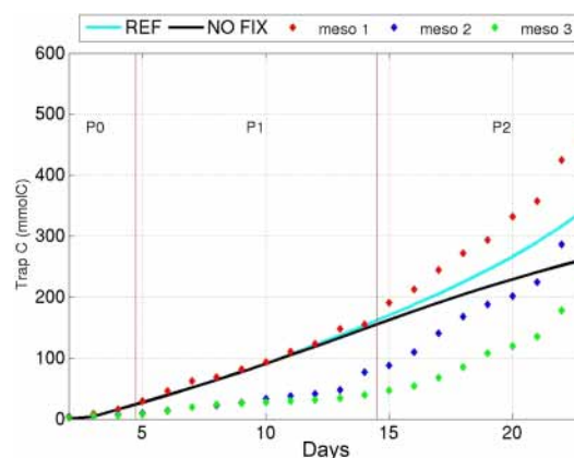
Figure 8. Evolution of C content collected in the mesocosm particle traps (mmol C) in the REF simulation (blue line) and the NOFIX simulation (black line; i.e. when the \text{N}_2 fixation process is removed).
