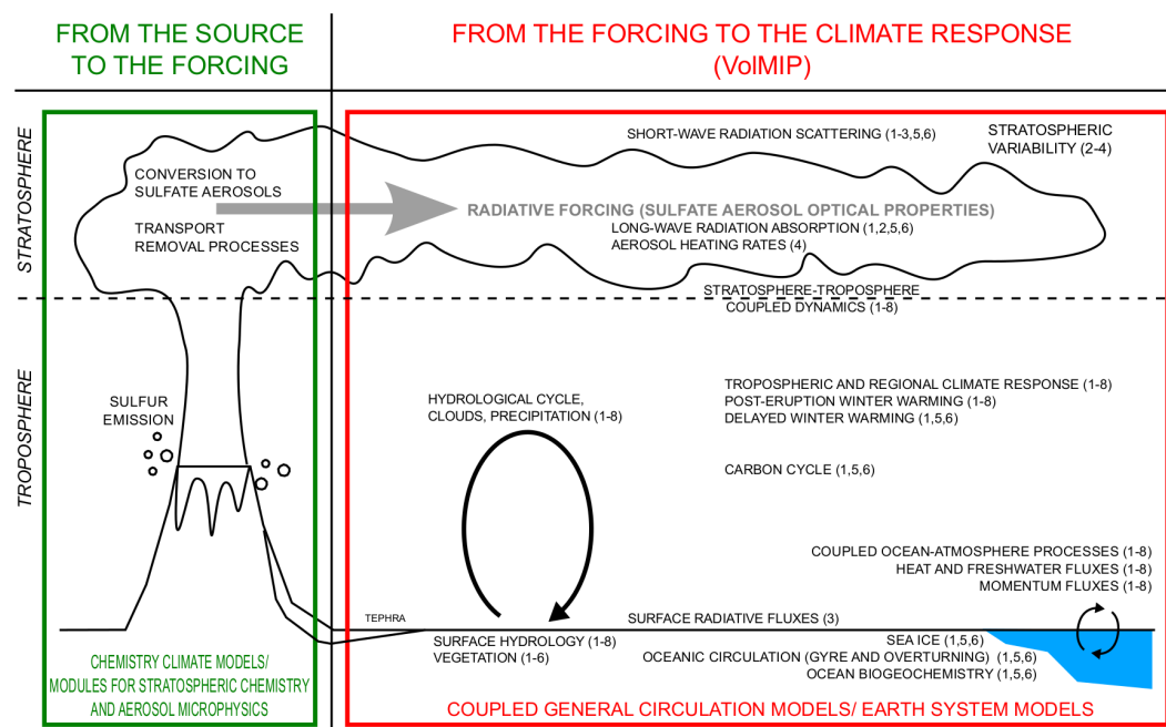
Figure 2. Illustrating the dominant processes linking volcanic eruptions and climatic response, with an overview of VolMIP experiments: 1 is volc-long-eq; 2 is volc-pinatubo-full; 3 is volc-pinatubo-surf; 4 is volc-pinatubo-strat; 5 is volc-long-hlN/hlS; 6 is volc-cluster-ctrl/-mill/-21C; 7 is volc-pinatubo-slab; 8 is volc-pinatubo-ini. The red box encompasses the processes related to the climatic response to volcanic forcing that are accounted for in VolMIP; the green box encompasses the processes regarding volcanic forcing that are neglected by VolMIP.
