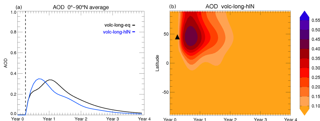
Figure 4. Consensus forcing for the volc-long-hlN experiment. (a) Northern Hemisphere average aerosol optical depth (AOD) at 550 nm produced by the Easy Volcanic Aerosol (EVA) module for a 56.2 Tg equatorial eruption (volc-long-eq, black line) and for a 28.1 Tg SO 2 Northern Hemisphere extratropical eruption (volc-long-hlN, blue line). (b) Time–latitude plots of the AOD at 550 nm from EVA for the 28.1 Tg SO 2 Northern Hemisphere extratropical eruption. The black triangle shows latitudinal position and timing of the eruption.
