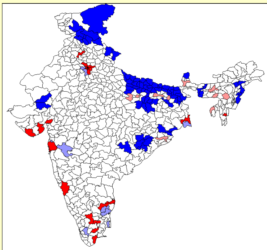
Hot spots, cold spots and spatial outliers
