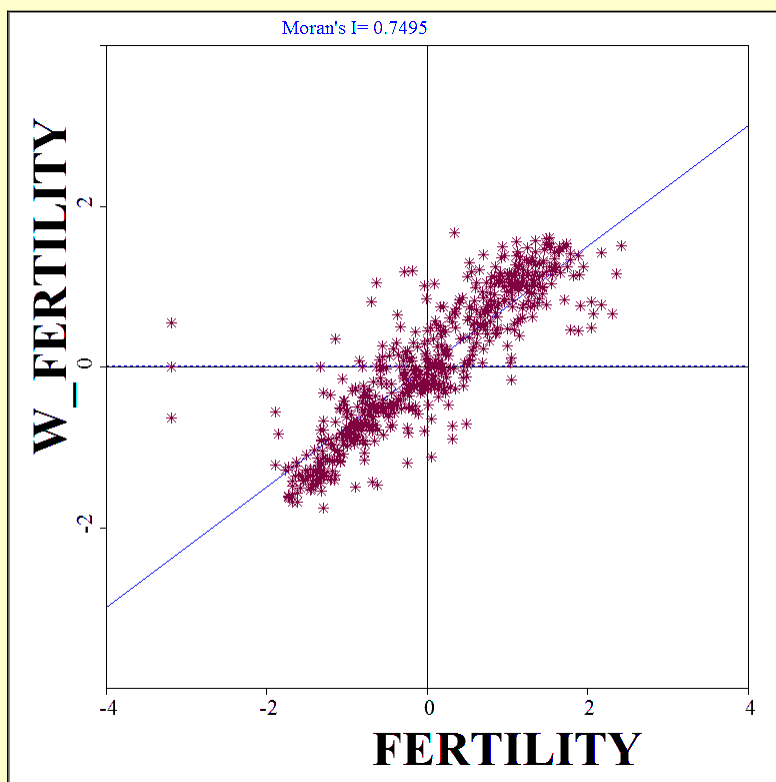
Moran scatterplot (observed values vs. spatial average of neighbours)
