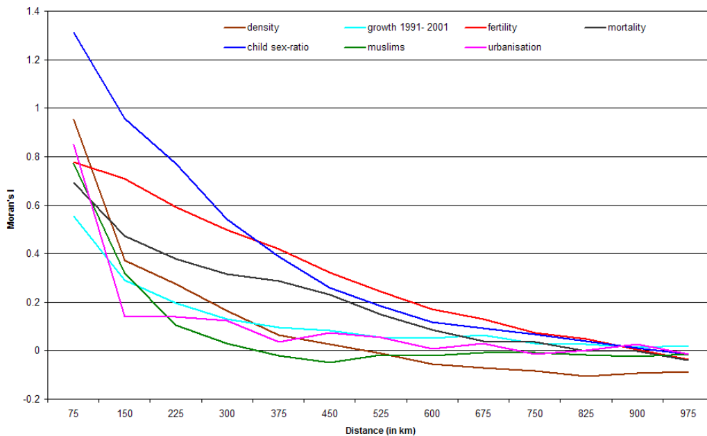
Figure 1: Moran's index (distance correlogram)
