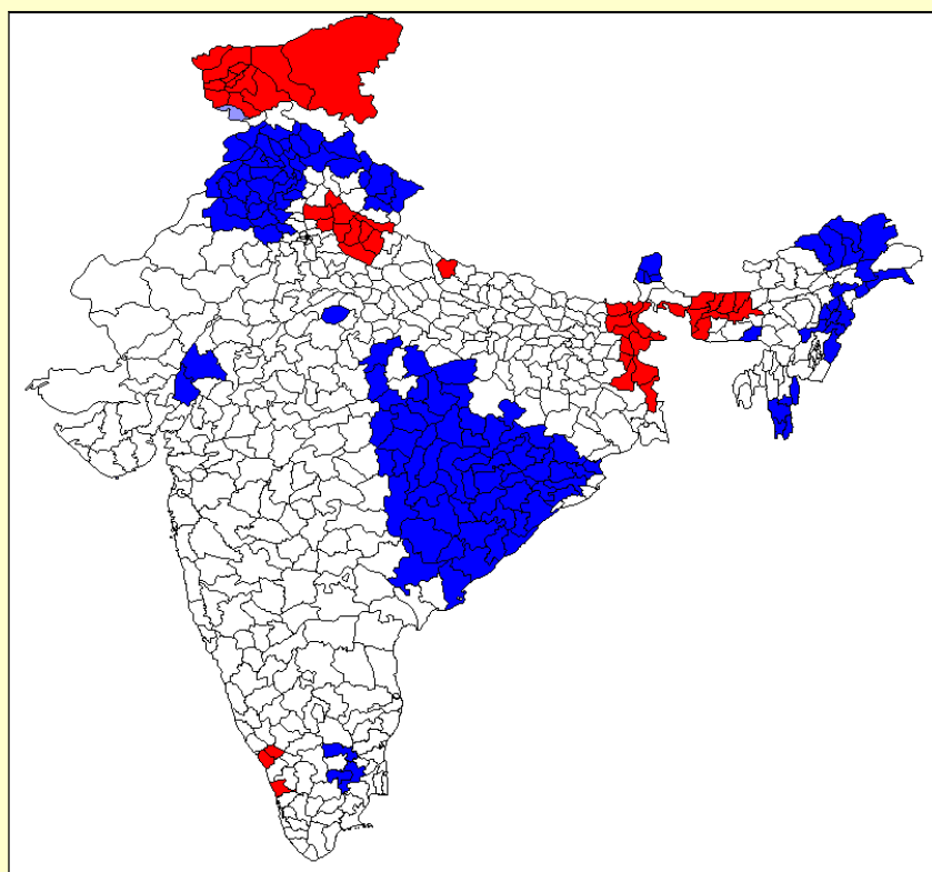
Hot spots, cold spots and spatial outliers
