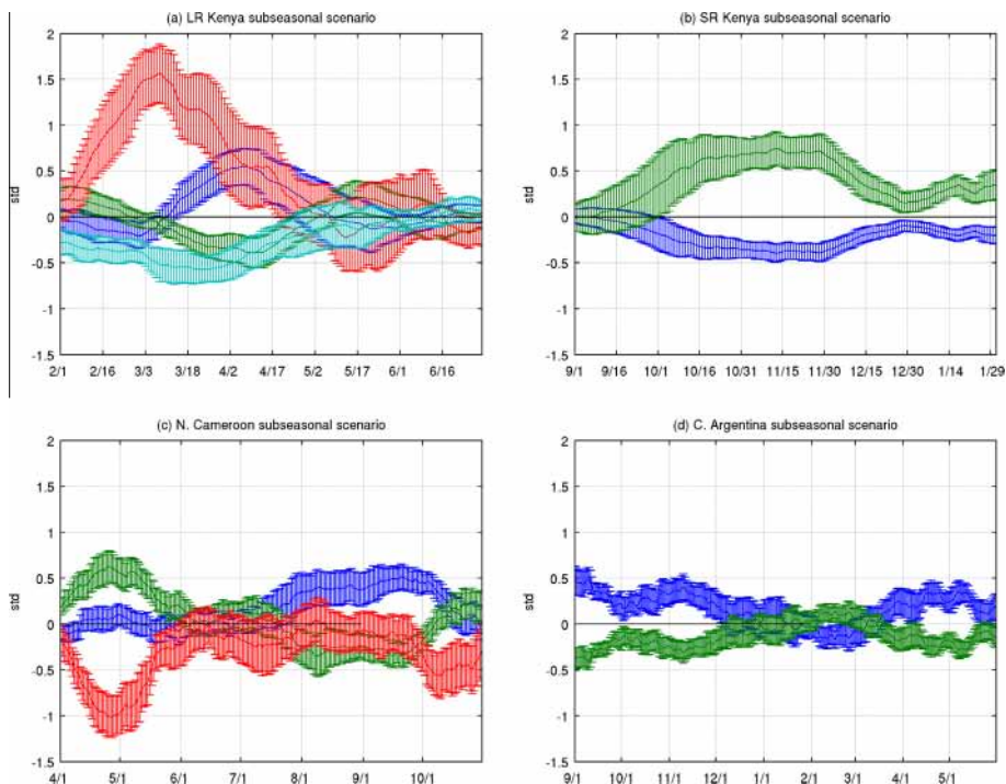
Fig. 9. Spatial average of standardized rainfall anomalies associated with the subseasonal scenarios (the error bars are +/- one standard deviation across stations).
