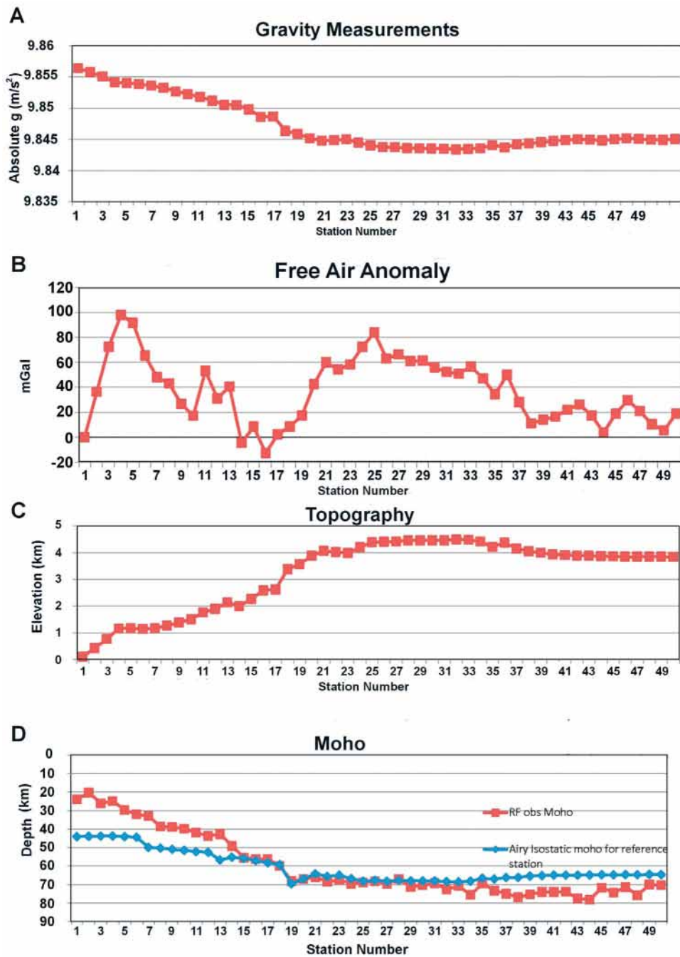
Figure 15. Results from a gravity survey performed along the seismic array by Caltech and UCLA students during a geophysical field course. (a) Observed absolute gravity ( m/s^2 ). (b) Free air anomaly (in mGal) relative to the first station, which shows an increase near the start of the line due to uplift near the coast. (c) Topography along the array. (d) Moho estimates from receiver function stacking and Moho depth estimates expected for Airy isostasy relative to a reference station.
