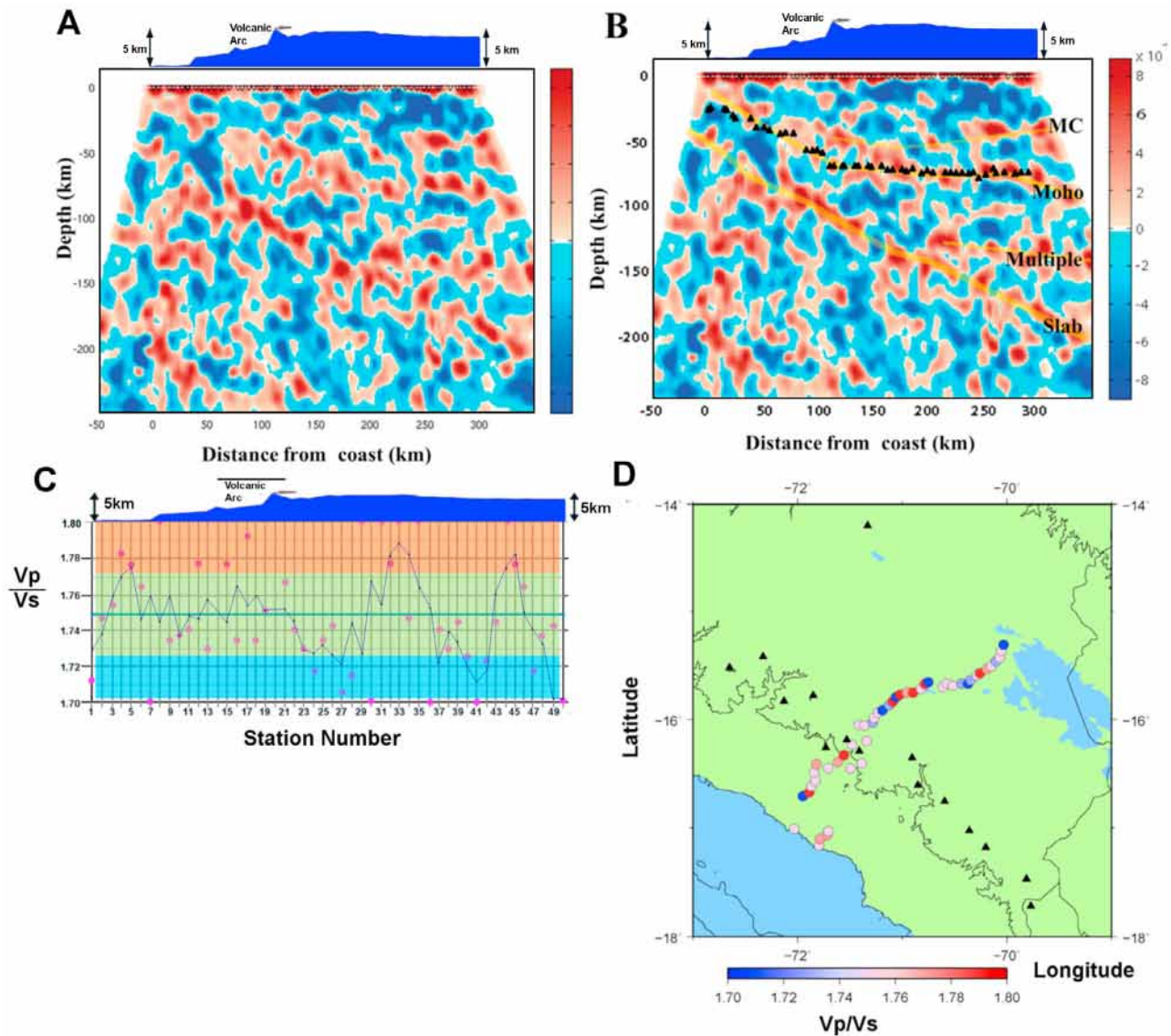
Figure 8. (a) Teleseismic P wave receiver function image based on events at a northwest azimuth to Peru with elevation along the array shown above. (b) Same image showing interpretation of the Moho, midcrustal structure, slab, and multiple of the midcrustal signal. Moho receiver function stacking results are plotted over the image. Elevation along the seismic line is shown above the image. (c) Average crustal V_p/V_s values ( y axis) versus station number (proxy for distance). Orange shading represents high V_p/V_s values, green shading represents midrange values, and light blue shading represents lower V_p/V_s values. The blue line shows the three-point running average of the V_p/V_s values. (d) Map of southern Peru showing a line with colors representing V_p/V_s ratios estimated from stacking of receiver functions. Black triangles represent active and dormant volcanoes in arc.
