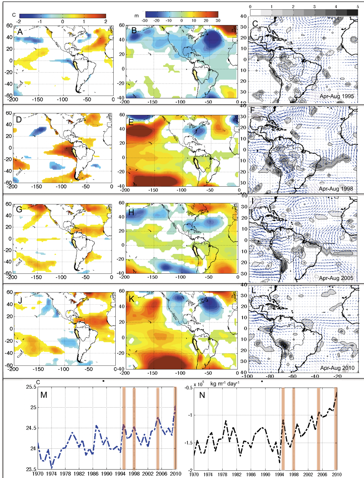
Figure 3. April to August mean SST (°C, left), 850 hPa geopotential height (m, centre) and vertically integrated water vapor flux anomalies (vectors, kg m -1 day -1 ) and positive divergence standardized values (contours, without unit) between the ground and 300 hPa (right) in (a–c) 1995, (d–f) 1998, (g–i) 2005, and in (j–l) 2010. Only values higher than 1 × standard deviation are plotted (2 × standard deviation for SST data). (m) Mean April–August SST in the 20°–60°W and 0°–30°N region and (n) mean April–August meridional water vapor flux between 0° and 15°S at 75°W.
