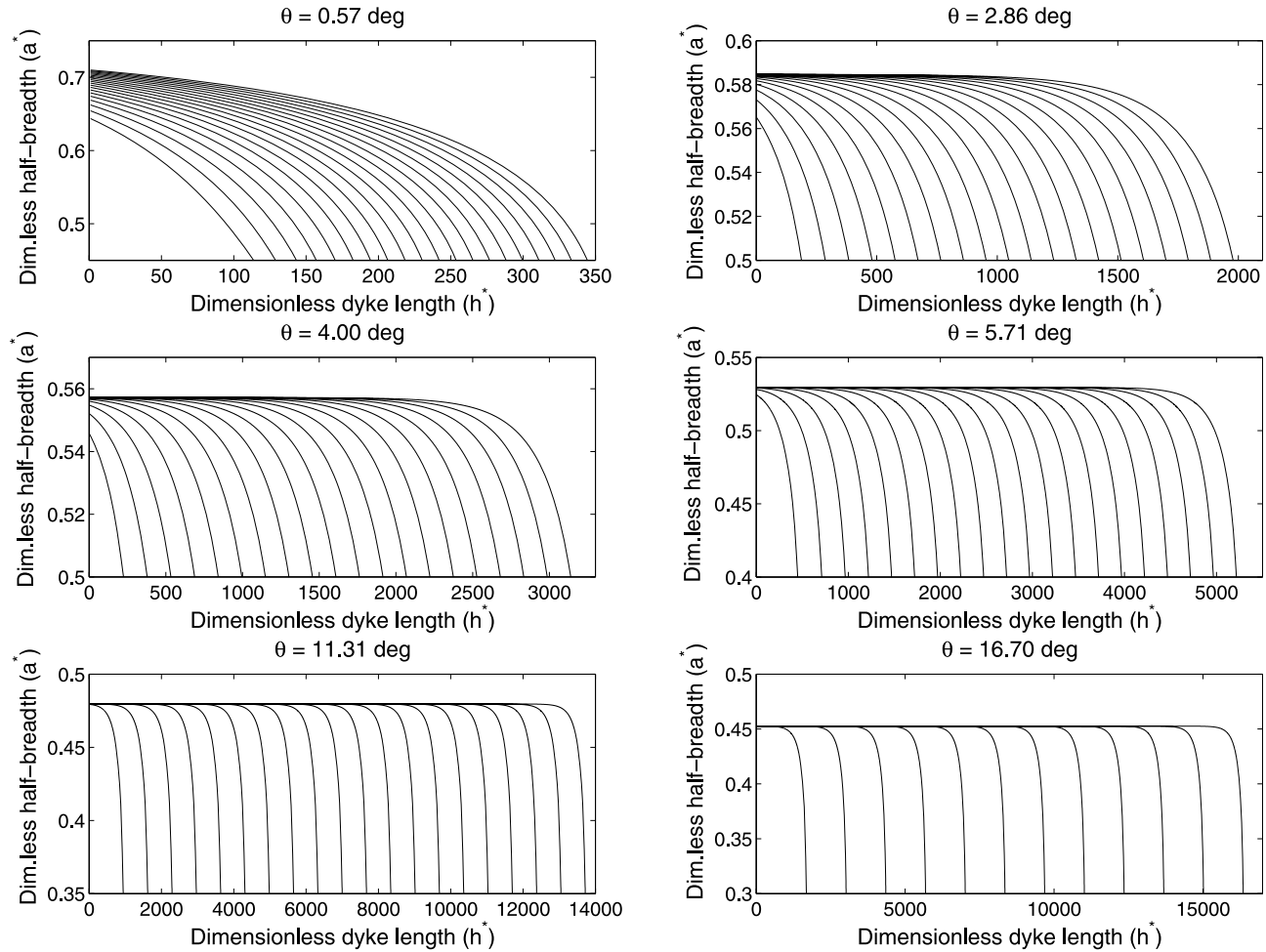
Figure 7. Lateral dike propagation: effect of the edifice flank slope on the fracture shape evolution over time. Parameters used in the calculations are \rho_{rl} = 2700 \text{ kg m}^{-3} , \rho_{ru} = 2300 \text{ kg m}^{-3} , \rho_m = 2400 \text{ kg m}^{-3} . Dimensionless time step between following curves is 10^{-6} . Dimensionless numbers values are N_1 = 1.65 \times 10^{-4} and N_2 = -1.48 \times 10^8 . N_1 = (3Q_{in}^{3/4} \mu^{3/4} G^{9/4}) / (H_b^{9/4} (1 - \nu)^{9/4} [P]^3) , N_2 = -(2H_b^3 (1 - \nu)^3 [P]^4) / (3\mu Q_{in} G^3) .
