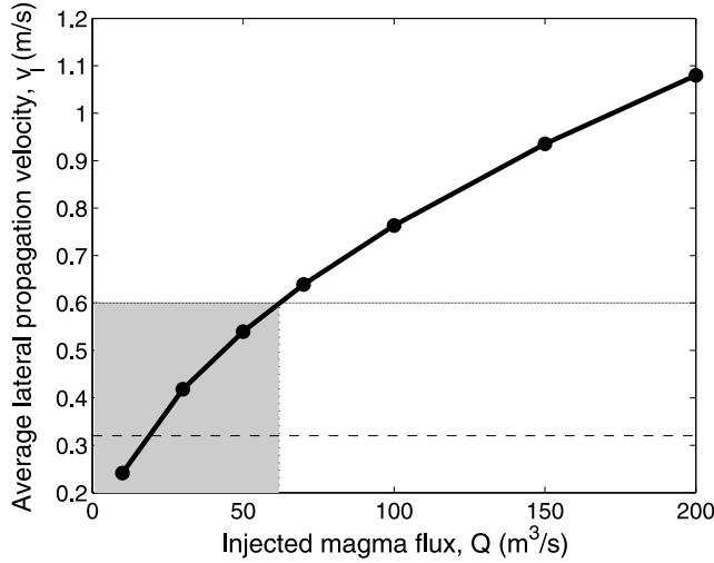
Figure 11. Lateral dike propagation: average propagation velocity versus influx of magma injected into the dike. Shaded area bounds the lateral propagation velocities estimated by Peltier et al. [2007] at Piton de la Fournaise. Parameters used are \theta = 11.8^\circ , \rho_{rl} = 2750 \text{ kg m}^{-3} , \rho_{ru} = 2300 \text{ kg m}^{-3} , \rho_m = 2400 \text{ kg m}^{-3} , H_b = 1150 \text{ m} , G = 1.125 \times 10^9 \text{ Pa} . Each magma flux value corresponds to a viscosity value, according to equation (40), where A = 4.3936 (from the vertical homogeneous case R_1 = -3.55 ). R_1 = (\rho_m - \rho_r)gH/\Delta P_0 .
