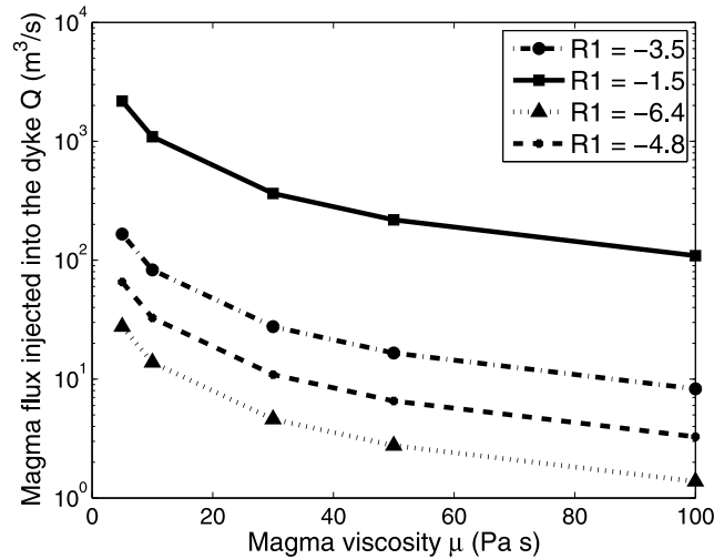
Figure 10. Dike rising vertically within a homogeneous medium from a constant overpressure magma reservoir. Magma flux injected into the dike as function of the magma viscosity and of the dimensionless number R_1 ( R_1 = (\rho_m - \rho_r)gH/\Delta P_0 ). Parameters used are H = 2250 m, \rho_m = 2400 kg m ^{-3} , \rho_r = 2750 kg m ^{-3} , a = 100 m, \nu = 0.25 , G = 1.125 \times 10^9 Pa.
