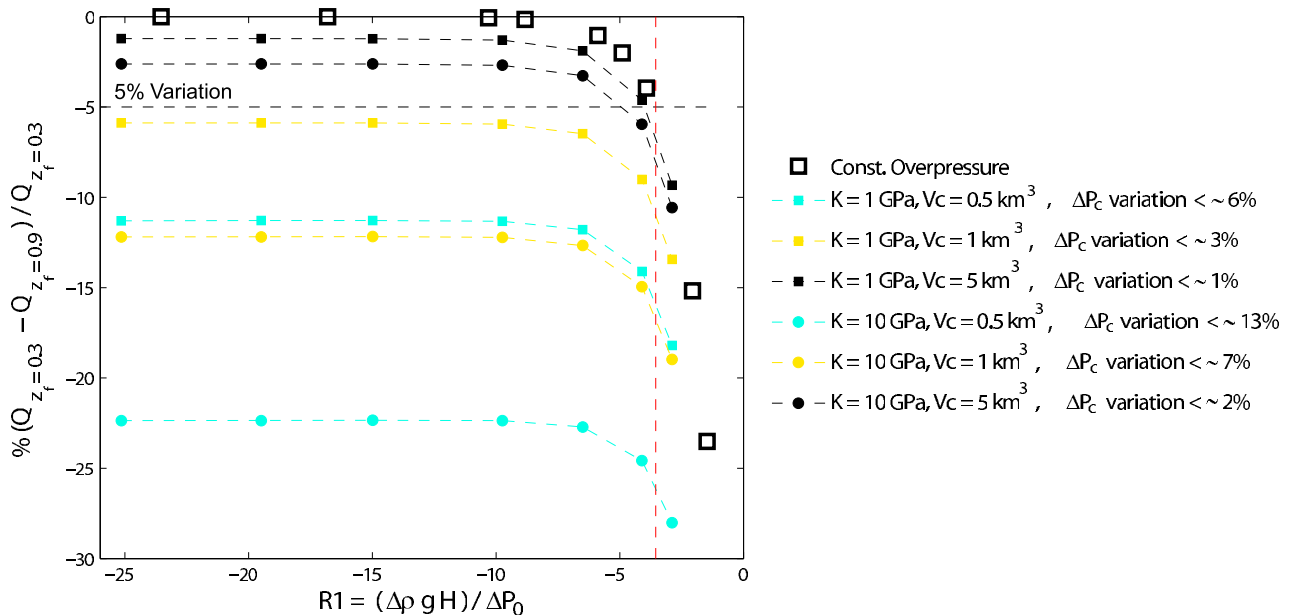
Figure 9. Interrelationship between magma influx and reservoir characteristics. Percentage of magma influx variation during dike growth within a homogeneous medium as function of the dimensionless number R_1 ( R_1 = (\rho_m - \rho_r)gH/\Delta P_0 ). Black squares indicate constant overpressure at the dike inlet; colored symbols indicate variable overpressure in the chamber. Colors are related to the V_c value; circles or squares depend on the K value. Reservoir overpressure variations \Delta P_c variation indicated in the legend are issued from the computation. Parameter values used are G = 1.125 \times 10^9 Pa, \nu = 0.25 , a = 100 m, g = 9.81 \text{ m s}^{-2} . V_c values derive from conceptual models of PDLF storage system [ Nercessian et al., 1996; Sapin et al., 1996; Peltier et al., 2007, 2008 ].
