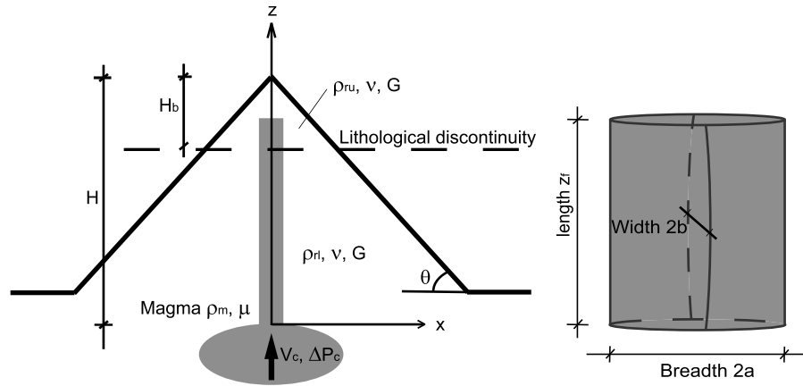
Figure 1. (left) Sketch illustrating the geometry of a vertical dike and (right) the shape of the fissure; 2b \ll 2a \leq z_f . Half breadth a is assumed a priori.
