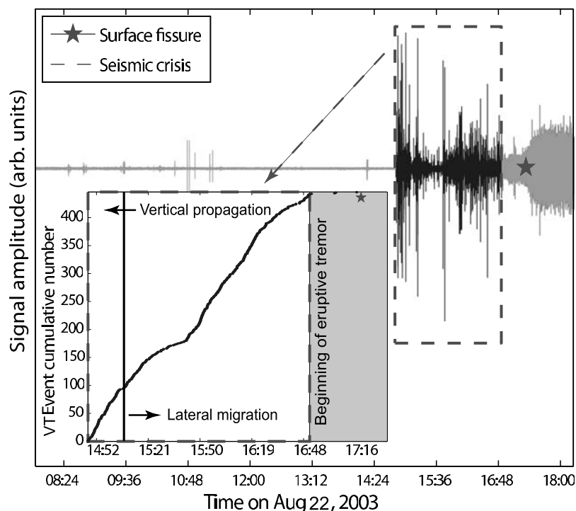
Figure 8. Seismic signal and cumulated seismicity (inset) hand-picked from continuous recordings recorded at the BOR summit station during the 22 August 2003 dike intrusion at Piton de la Fournaise volcano. Times related to the different stages of activity are from Peltier et al. [2007].
