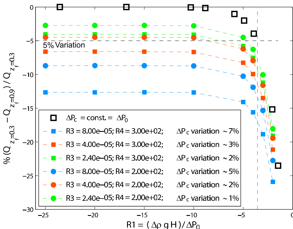
Figure 3. Percentage of magma influx variation during dike growth within a homogeneous medium as function of the dimensionless number R_1 ( R_1 = (\rho_m - \rho_r)gH/\Delta P_0 ). Black squares indicate constant overpressure at the dike inlet; colored symbols indicate variable overpressure in the chamber. Color of solid symbols is related to the V_c value; circles or squares depend on the K value. Reservoir overpressure variations \Delta P_c variation indicated in the legend are issued from the computation.
