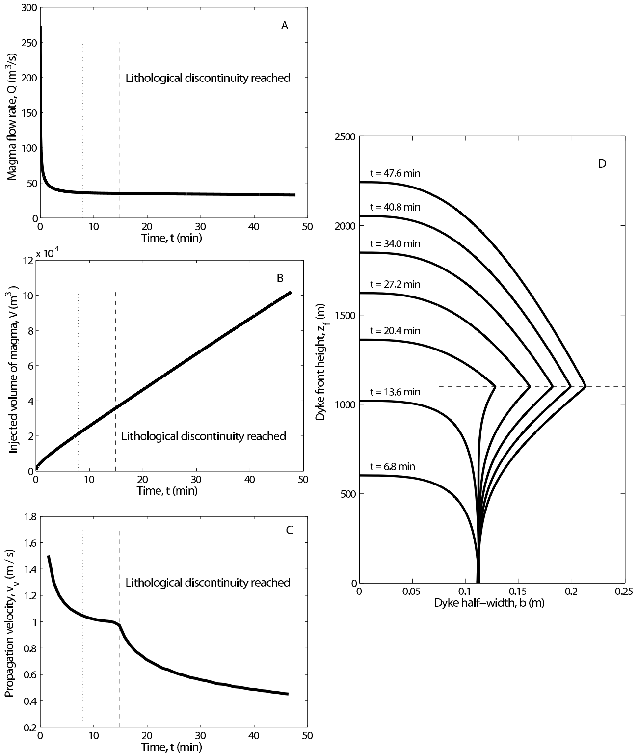
Figure 13. Effect of a lithological discontinuity on the vertical propagation of a magma-filled dike. (a) Magma flux injected into the dike over time; (b) dike volume (i.e., cumulative volume of magma injected into the dike over time); (c) propagation velocity versus time; (d) evolution of the crack shape for progressive growth stages. Parameter values used in the calculation are listed in Table 2. Dotted lines in Figures 13a, 13b, and 13c correspond to z_f/H = z_f^* = 0.3 .
