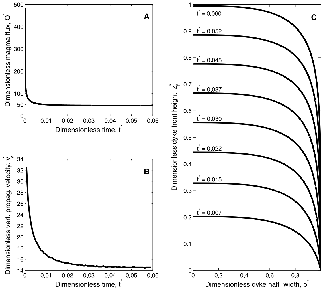
Figure 2. Magma-filled dike rising in a homogeneous medium from a constant overpressure magma chamber at depth. (a) Dimensionless magma flux injected into the dike over time; (b) dimensionless propagation velocity versus time; (c) evolution of the crack shape for progressive growth stages. R_1 ( R_1 = (\rho_m - \rho_r)gH/\Delta P_0 ) value used in the calculation is -3.55 . Dotted lines in Figures 2a and 2b indicate z_f = 0.3 . Here t = t^*[t] , Q = Q^*[Q] , v_v = v_v^*[v] , b = b^*[b] , z_f = z_f^*[H] , where scales for time [t] , flux [Q] , and fracture width [b] are given in equations (6) to (8); lengths are scaled by the reservoir depth H ; and scale for propagation velocity is [v] = [H]/[t] .
