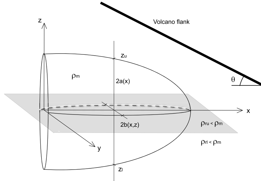
Figure 6. Sketch illustrating the geometry and the main parameters of a dike horizontally propagating at the level of neutral buoyancy.
