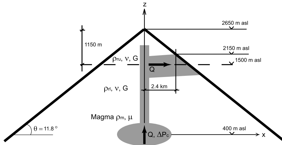
Figure 12. August 2003 PDLF case study. Sketch illustrating the geometry used in the model. Dashed line indicates input lithological discontinuity, position from Peltier et al. [2007]. Gray zones indicate magma path. All elevation data come from Peltier et al. [2007].
