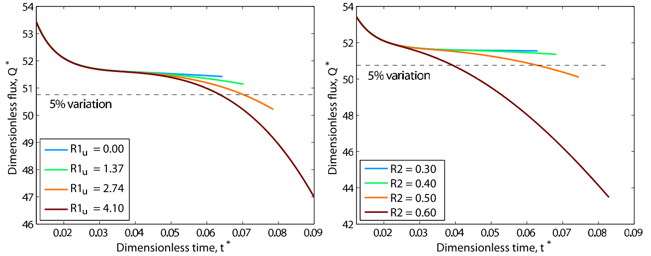
Figure 5. (left) Effect of the dimensionless number R_{1ru} on the magma flux evolution over time during dike propagation, R_2 = 0.43 . (right) Effect of the dimensionless number R_2 on the magma flux evolution over time during dike propagation, R_{1ru} = 1.37 . For both cases, R_{1rl} = -4.1 , V_c = 5 \text{ km}^3 and K = 1 \times 10^9 \text{ Pa} . Final time corresponds to surface attainment. R_{1u} = (\rho_m - \rho_{ru})gH/\Delta P_0 , R_{1l} = (\rho_m - \rho_{rl})gH/\Delta P_0 , R_2 = H_b/H , R_3 = (\Delta P_0 a^2 (1 - \nu) H) (GV_c) , R_4 = 4KG/(\Delta P_0(4G + 3K)) .
