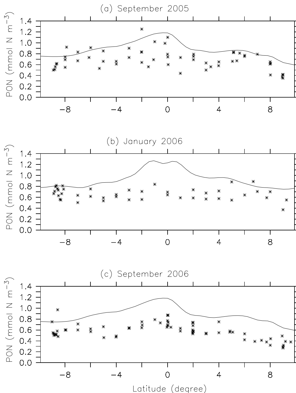
Fig. 4. Modeled (lines) versus measured (symbols) surface concentrations of PON (140° W–125° W) in (a) September 2005, (b) January 2006, and (c) September 2006.
