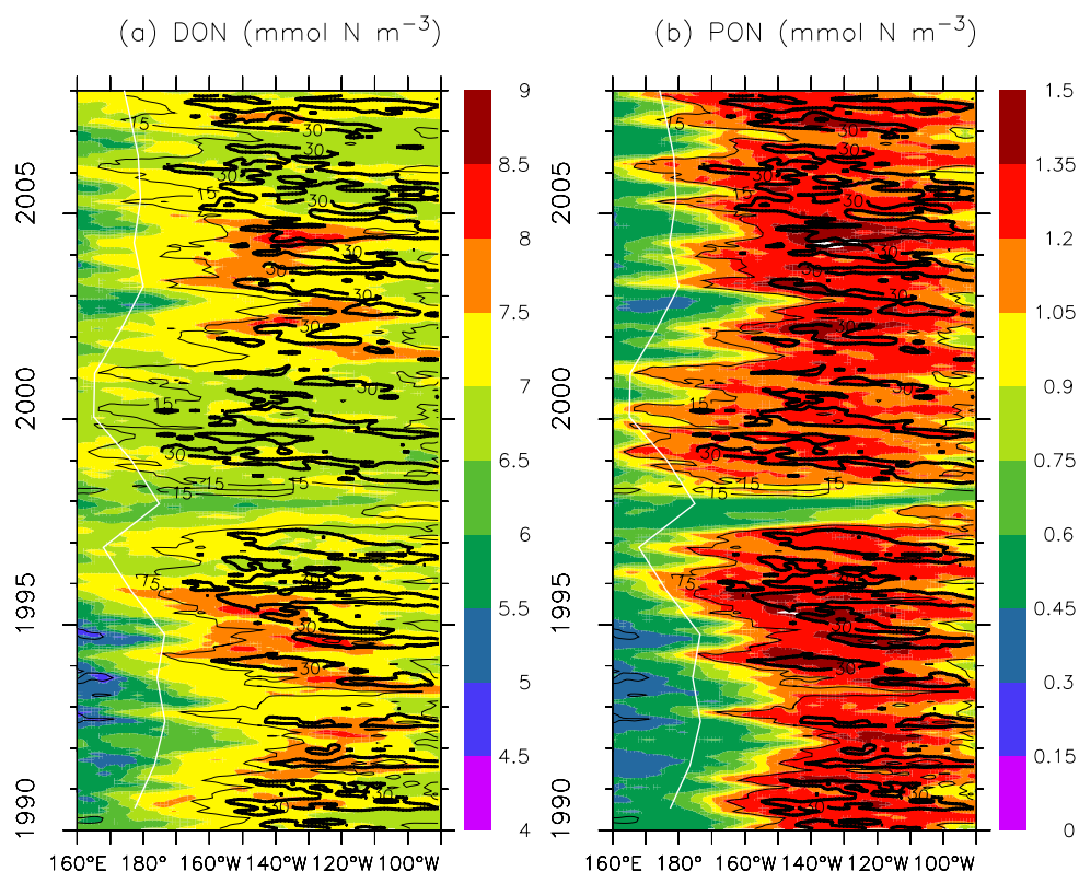
Fig. 9. Time-longitude contours of (a) DON (color contour) and iron concentrations (black lines), and (b) PON (color contour) and iron concentrations (black lines) averaged over the 5° N–5° S band. Superimposed white lines denote the longitude of HNLC front (173.2–10.75 SOI).
