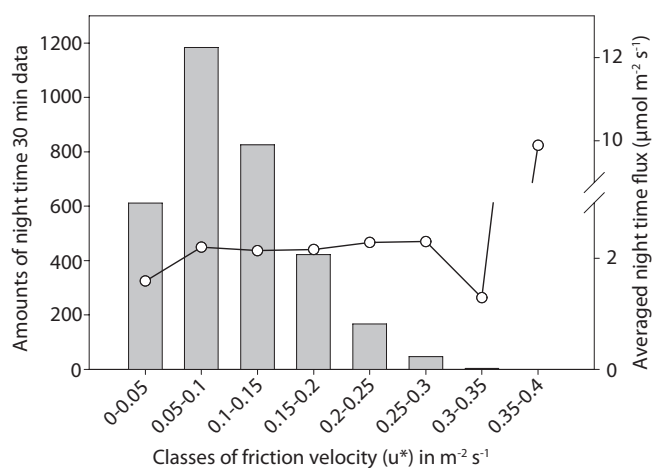
Fig. 2. An example, showing how u^* thresholds were defined, from grassland site at Tchizalamou, the Republic of Congo. The left y-axis shows the number of 30 min intervals for each u^* class and the right y-axis shows the averaged flux for each class. For u^* < 0.05 , the average flux is depressed. We rejected these data as they lead to underestimation. For 0.05 < u^* < 0.3 the average flux is stable and used in the analysis. For u^* > 0.3 averaged fluxes are exaggerated, leading to overestimation, and were rejected.
