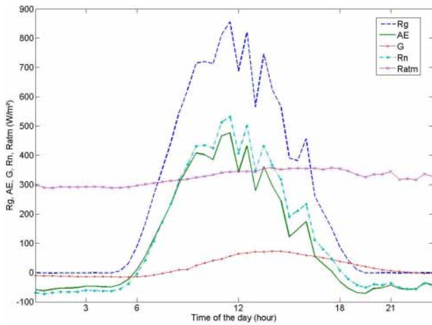
Fig. 2. Illustration of the typical course of AE, R_g , G , R_n and R_{atm} during a day (doyle 124, Auradé 2006).
