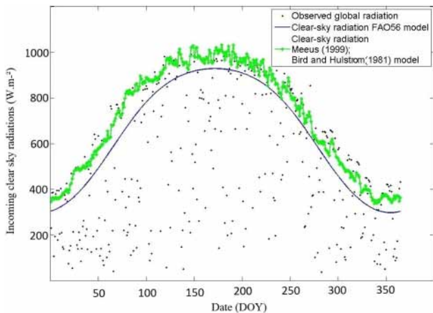
Fig. 3. Observed vs. estimated clear sky radiations at noon using FAO and combined Meeus and Bird and Hulstrom model for Lamasquère 2007.
