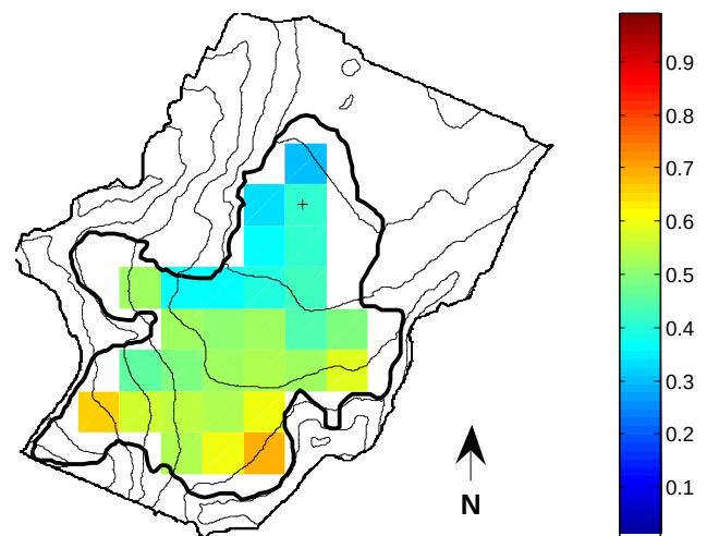
Fig. 4. Clear sky albedo retrieved from MODIS on 16 July 2007. This map has been retrieved using anisotropic/topographic corrections and DISORT. The pixel indicated by the plus is the pixel used for the monitoring of the albedo in the ablation zone. All the coloured pixels are used to compute the mean albedo of the glacier.
