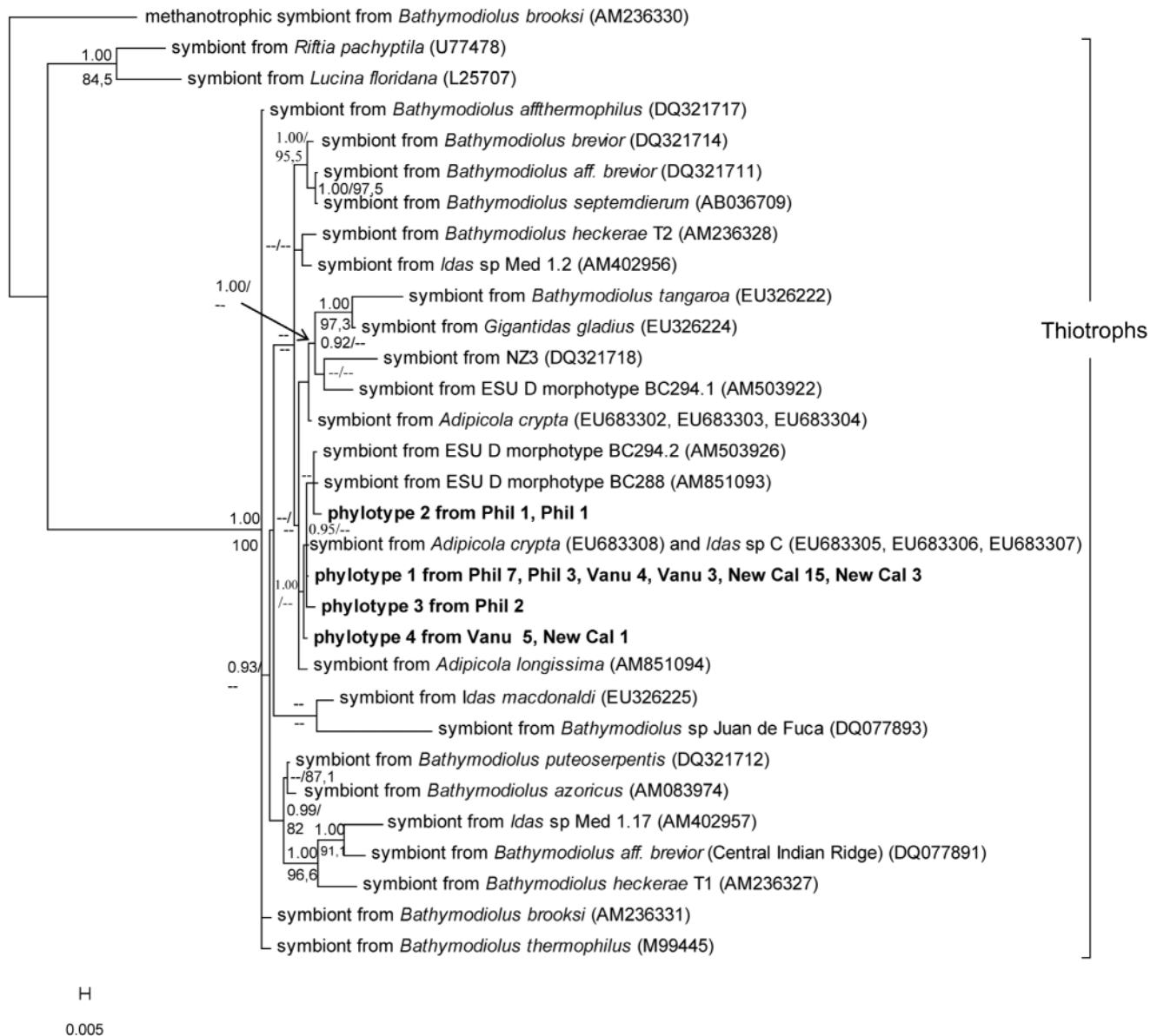
Figure 6. Bayesian tree displaying bacterial symbionts based on the analysis of the 16S rRNA. Phylotypes associated with I. iwaotakii are shown in bold. Posterior probabilities (PP) and bootstrap values obtained from ML analysis are given above and below branches respectively. PP and bootstrap values lower than 0.90 and 50%, respectively, are not shown. The scale bar represents 0.5% estimated base substitution. doi:10.1371/journal.pone.0069680.g006
