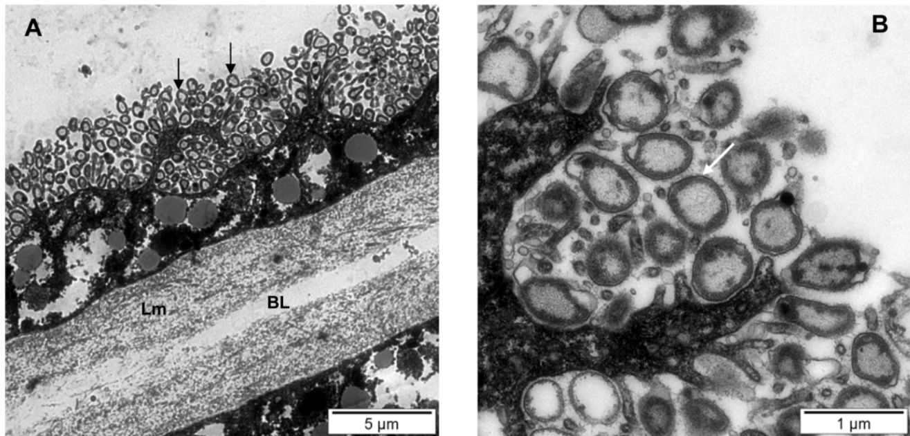
Figure 7. Gill filaments of Idas iwaotakii . (A) TEM view of gill filament of the lateral zone from a specimen of I. iwaotakii collected on wood off Vanuatu. Bacteria (black arrows) are located extracellularly in contact with microvilli. BL: blood lacuna; Lm: basal lamina. (B) Electron micrograph of the extracellular symbionts. Symbiotic bacteria possess a double membrane (white arrow) typical of Gram negative bacteria. doi:10.1371/journal.pone.0069680.g007
