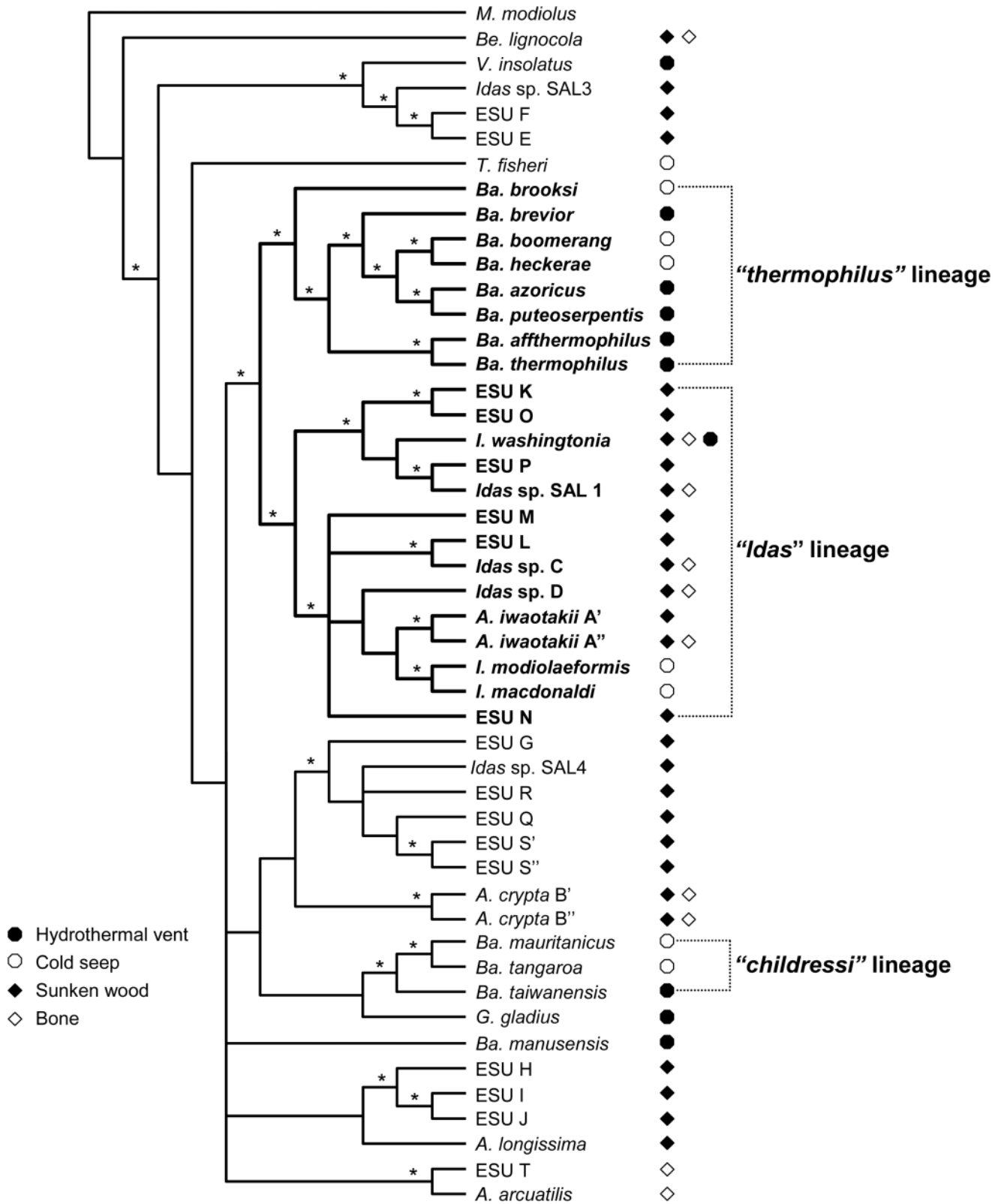
Figure 1. Dendrogram obtained from Bayesian analyses of the combined dataset of COI mtDNA and the 28S rRNA. Asterisks correspond to nodes with posterior probabilities (PP) obtained from BA analysis and bootstrap values obtained from ML analysis that are higher than 0.90 and 50%, respectively. (modified from [7]). doi:10.1371/journal.pone.0069680.g001
