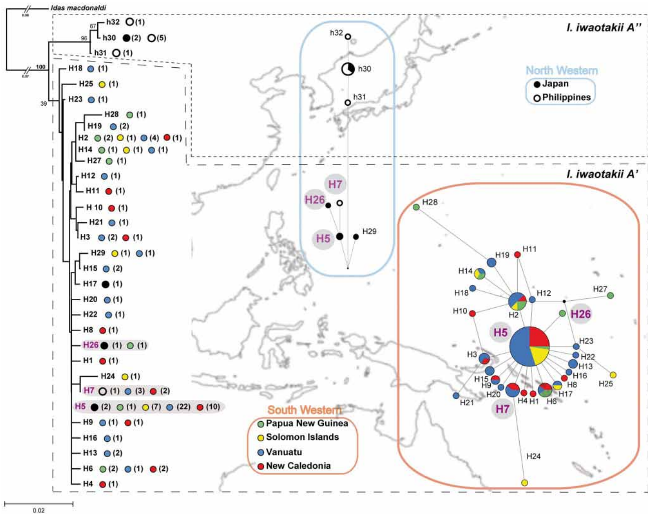
Figure 3. Population structure of I. iwaotakii . Left part: K2P neighbour-joining tree of unique COI haplotypes of I. iwaotakii . The localities at which each haplotype have been sampled is figured by a coloured circle (see legend for correspondence between localities and colours), the number of individuals sharing the same COI haplotype at each locality is given in brackets. The grey rectangles underline the haplotypes shared by the two studied regions. The scale bar represents 0.02% estimated base substitutions. The mitochondrial haplotypes of I. iwaotakii are divided in two clades, A' and A'', represented by one panel with large dots and the other one with small dots, respectively. Right part: Median-joining networks (MJN) from COI mtDNA data drawn independently for each of the two studied regions (North Western and South Western haplotypes). Size of haplotype circles is proportional to the number of specimens. Colours used to figure the localities within each region are the same of that used for the NJ tree. A small black circle represents a hypothetical haplotype. The haplotypes shared by the two studied regions are underlined using grey circles over haplotype labels.
