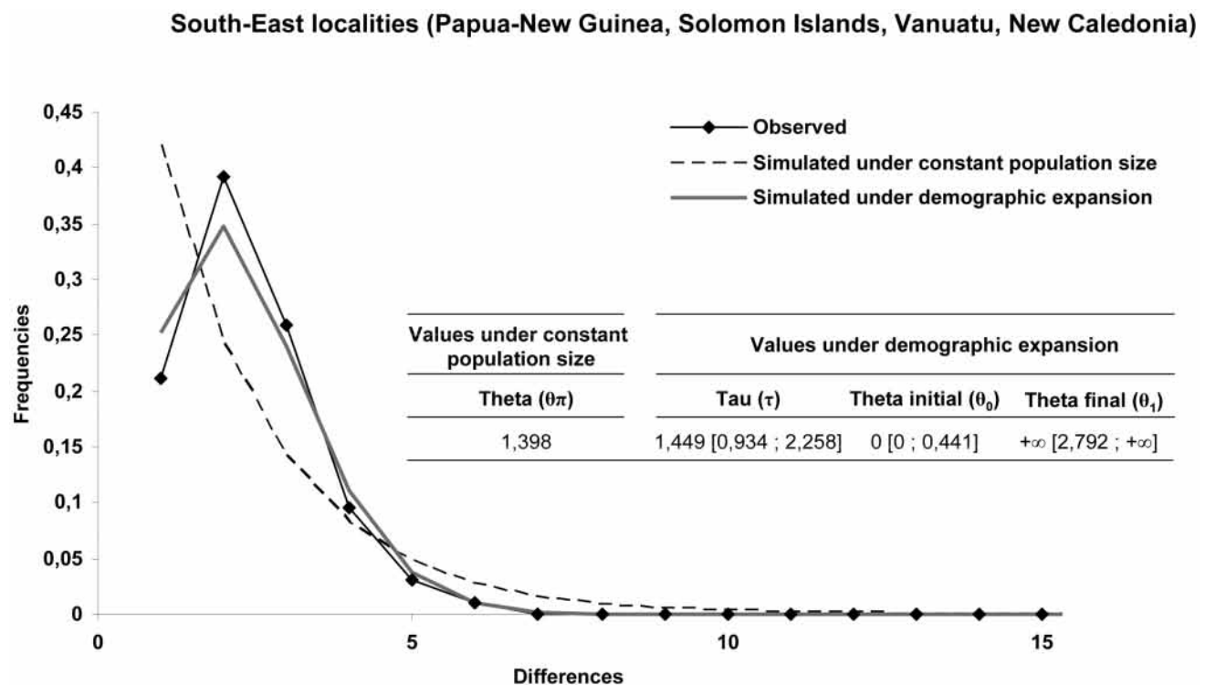
Figure 4. Mismatch distributions of COI haplotypes. COI haplotypes observed, simulated under a constant population size and a model of population expansion for the South-west Pacific populations of A. iwaotakii . Along x-axis are indicated the numbers of nucleotide differences between all pairs of sequences and on y-axis the frequencies of pairs. The table summarizes the parameters of demographic analyses under constant population size and demographic expansion. The confidence intervals at 99% of the parameters under a demographic expansion model are given in square brackets. doi:10.1371/journal.pone.0069680.g004
