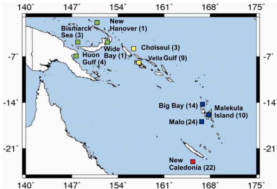
Figure 2. South Western Pacific map showing the sampling localities of mussels of Idas iwaotakii . Specimens from Malo and New Caledonia have already been studied by [7,30]. doi:10.1371/journal.pone.0069680.g002
