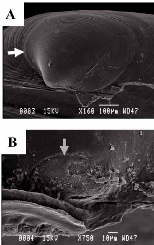
Figure 5. Scanning electron micrographs of the larval shell of a specimen of Idas iwaotakii . Pictures: (A) Dorsal view showing prodissoconch I (PI) and prodissoconch II (PII); the white arrow indicates the boundary between the dissoconch and prodissoconch, (B) Detail of PI; the grey arrow indicated of the boundary between PI and PII. doi:10.1371/journal.pone.0069680.g005
