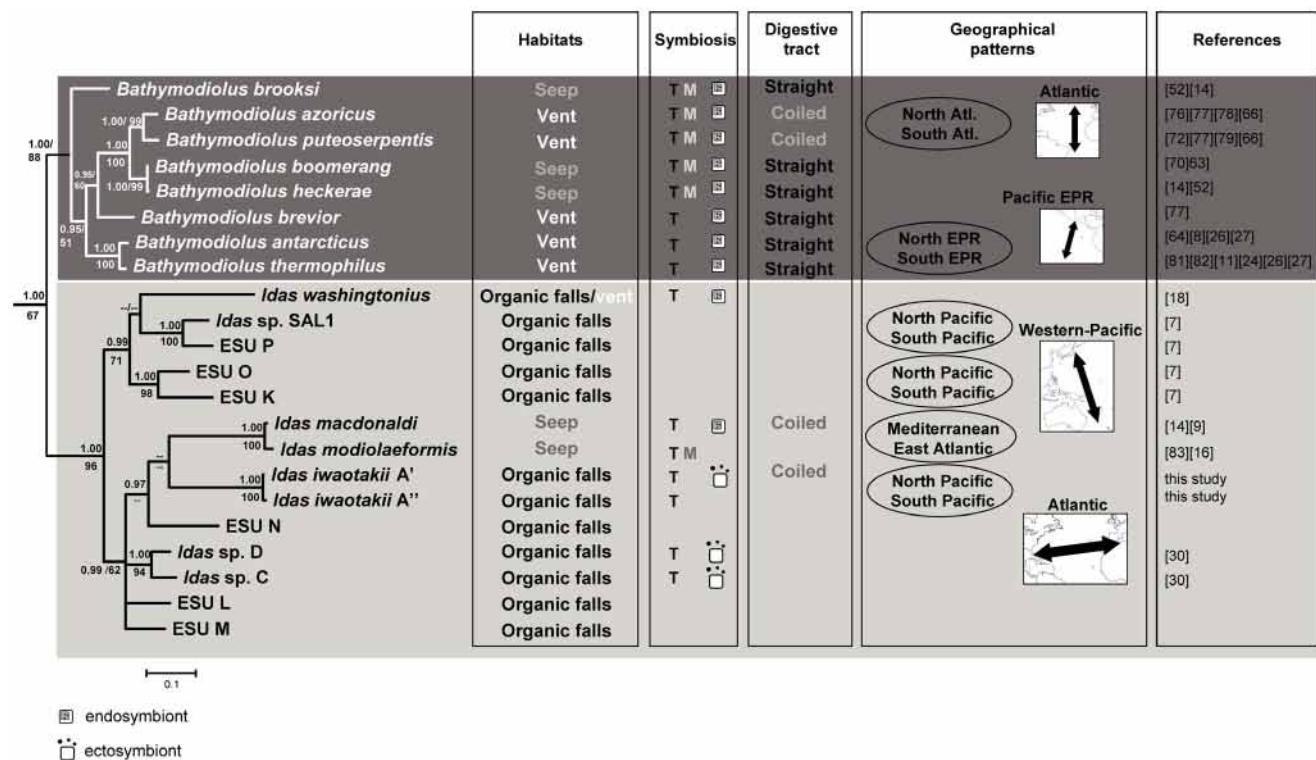
Figure 9. Comparison of data available for the “thermophilus” lineage and its sister lineage. The “thermophilus” lineage is represented by the dark grey rectangle and its sister lineage, corresponding to the genus Idas , by the light grey rectangle. Phylogenetic relationships correspond to a part of the combined COI mtDNA and 28S rRNA phylogenetic tree from [7]. T: thiotrophic symbiont; M: methanotrophic symbiont. In geographical patterns section, the ovals correspond to pairs of sister-species with an allopatric distribution and location maps illustrate the allopatric distribution of these sister pairs. References: [7–9], [11], [14], [16], [24], [26–27], [30], [52], [63–64], [66], [70], [72], [76–83]. doi:10.1371/journal.pone.0069680.g009
