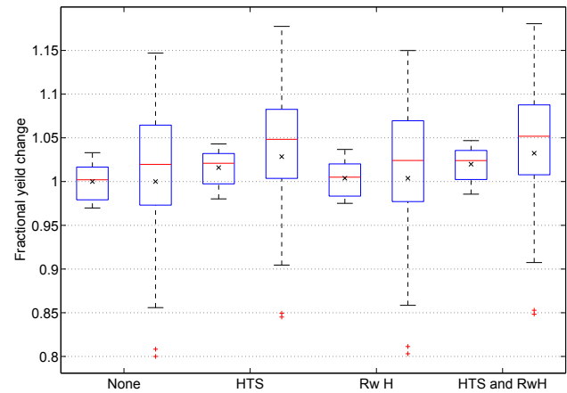
Figure 6. Efficacy of adaptation methods for maize in GLAM. HTS is crops adapted to high-temperature stress, Rw H shows crops with rainwater harvesting, and HTS and Rw H shows both adaptation methods in use. Each box shows the fractional yield change relative to the unadapted crop with the box plots showing the range across the six-member GCM–RCM ensemble. The pairs of boxes show the relative change in yield for the adaptation method in the historic climate (left) and the future climate (right).
