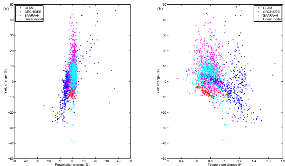
Figure 5. Percentage maize yield change against precipitation (a) and temperature (b) for four crop models. This figure has a restricted x axis in the precipitation plot to enhance the clarity of the results and a full version is shown in Fig. S2.
