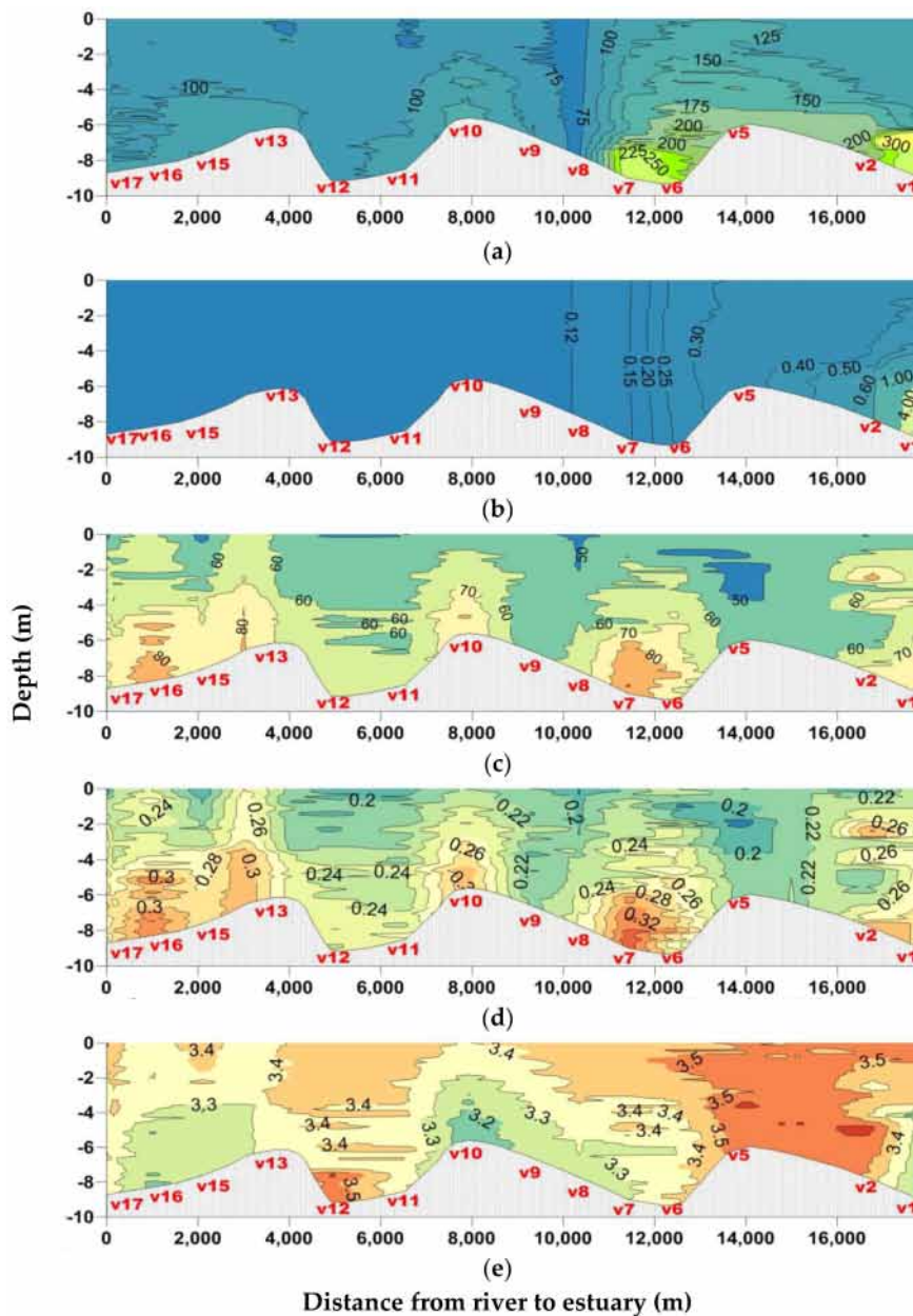
Figure 3. 2D distributions of parameters along Transect 1 during flood tide (water elevation = 1.3–2.5 m, 10 May 2015). (a) Turbidity (FTU); (b) Salinity (psu); (c) D_{50} in the whole grain size range (1.48–212 \mu\text{m} ); (d) Settling velocity of flocs ( \text{mm s}^{-1} ); (e) PSD slope.
