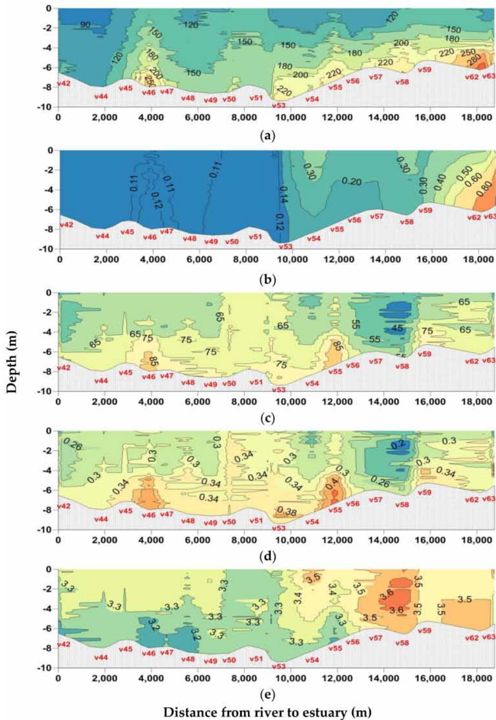
Figure 7. 2D distributions of parameters along Transect 4 during low tide (water elevation = 0.7–0.8 m, 12 May 2015). (a) Turbidity (FTU); (b) Salinity (psu); (c) D 50 in the whole grain size range (1.48–212 μm); (d) Settling velocity of flocs (mm s -1 ); (e) PSD slope.
