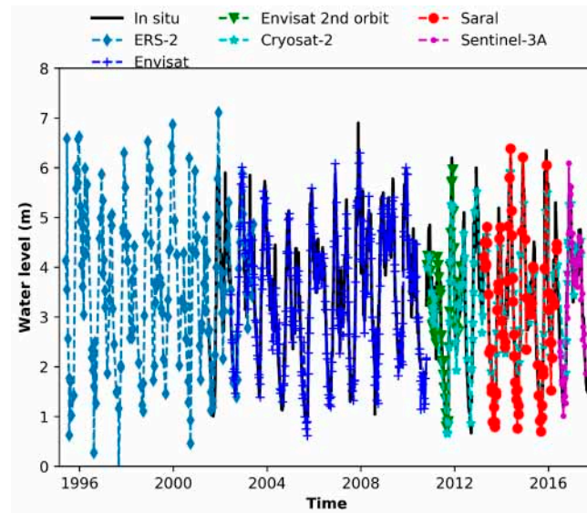
Figure 10. Time series of water level at Lambaréné from the in-situ gauge record (black continuous line), the multi-mission altimetry-based record (ERS-2 data are represented with diamonds, ENVISAT with blue crosses on its nominal orbit and with green triangles on its second orbit, Cryosat-2 with green-blue stars, SARAL with red circles, Sentinel-3 with purple dots).
