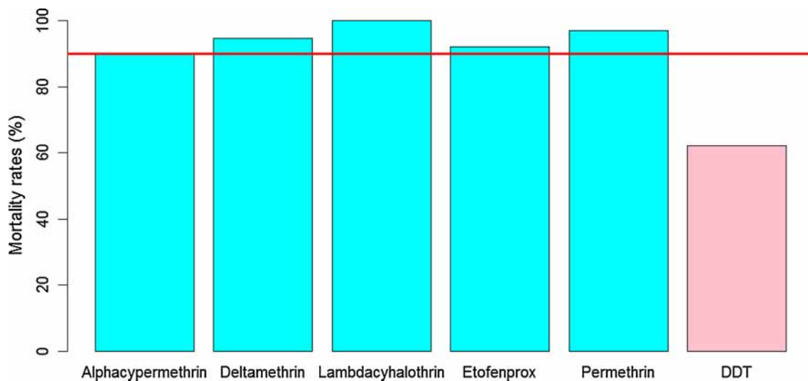
Fig. 2 Mortality rates of Anopheles gambiae s.l. from Dielmo, after exposure to pyrethroids (alphacypermethrin 12.5 µg/bottle, deltamethrin 12.5 µg/bottle, etofenprox 12.5 µg/bottle, lambdacyhalothrin 12.5 µg/bottle, permethrin 21.5 µg/bottle) and DDT 100 µg/bottle (organochlorine). Percentage mortality was plotted after exposure at DT of each insecticide. The horizontal line indicates a 90% resistance threshold according to WHO criteria. Pyrethroids are represented by blue bars and organochlorine by pink bars
