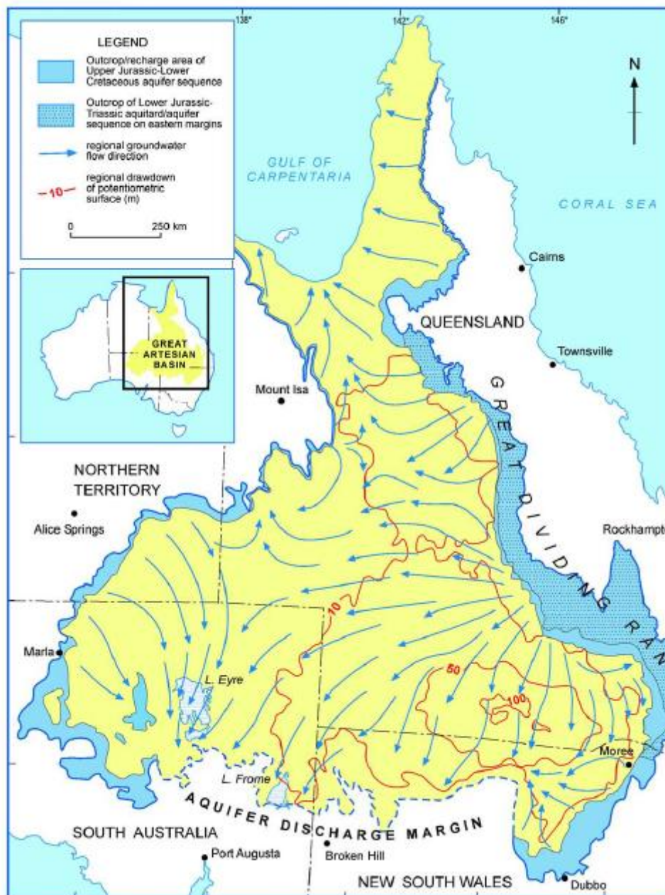
Figure 59. The Great Artesian Basin of Australia
