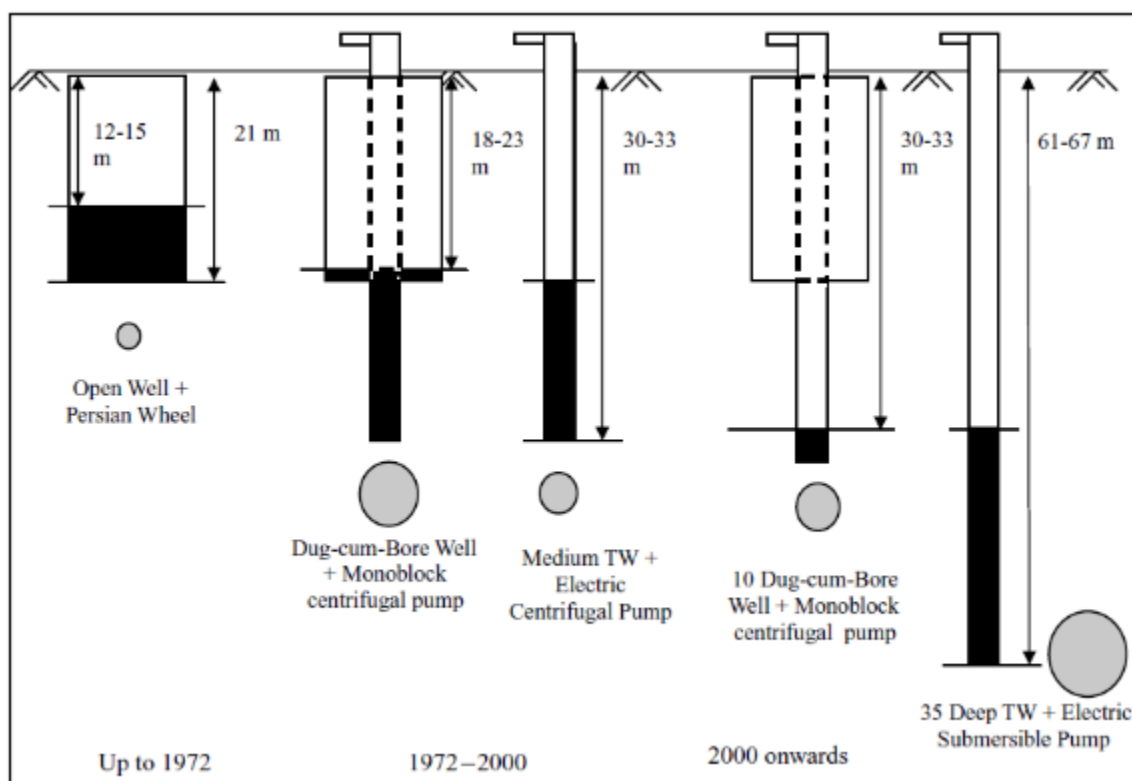
Figure 18. Evolution of tubewell technology in Bajjal village, Punjab, North India
