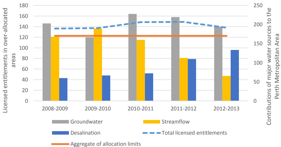
Figure 57. Licensed entitlements in the Gnangara Groundwater system and contributions from major water sources to the Perth Metropolitan Area water supply
