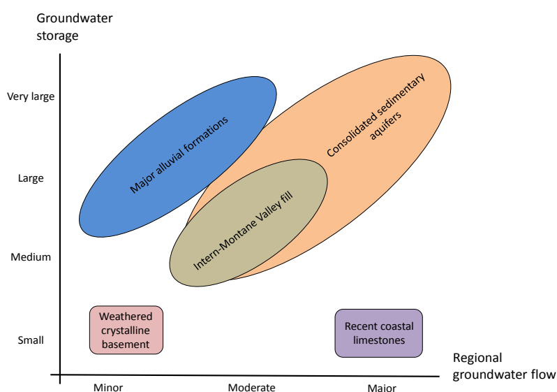
Figure 15. General aquifer types
