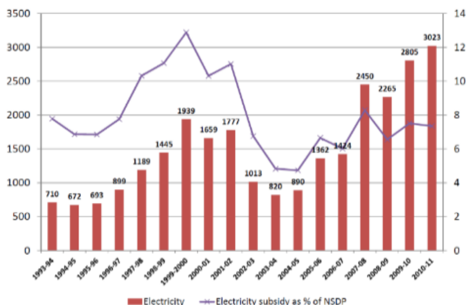
Figure 36. Trends in power subsidy in Punjab (RS 10 millions)
