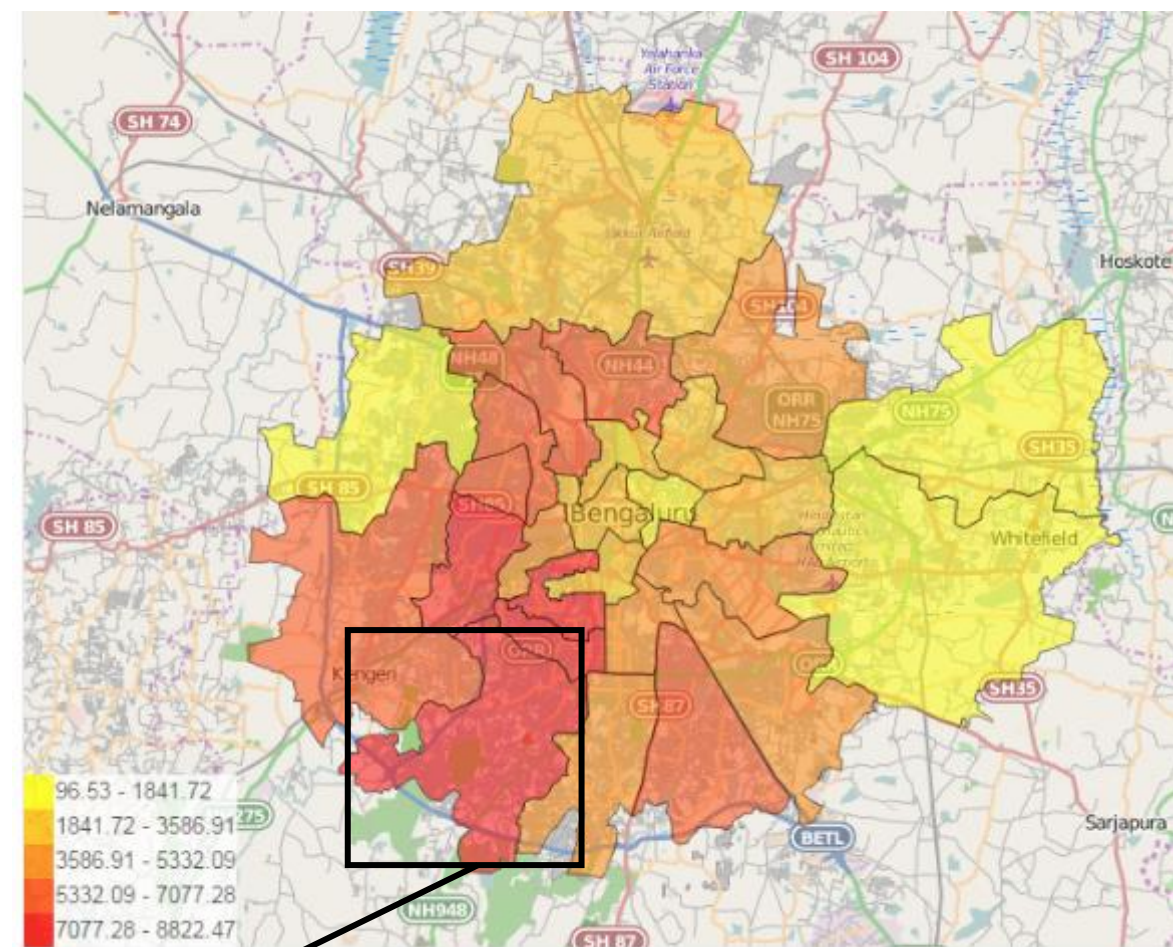
Figure 30. Estimated average borewell density in Bangalore
