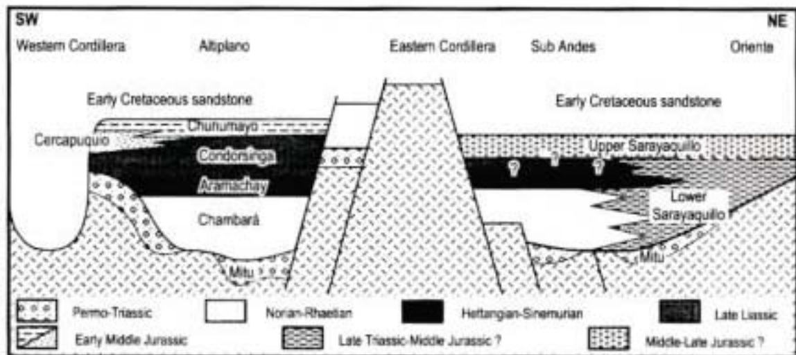
FIGURE 12 - Paleogeographic sketch of the Pucara Group (Late Triassic-Early Middle Jurassic) of Central Peru (after Rosas and Fonthoté, 1995). Compare with Fig. 11.
