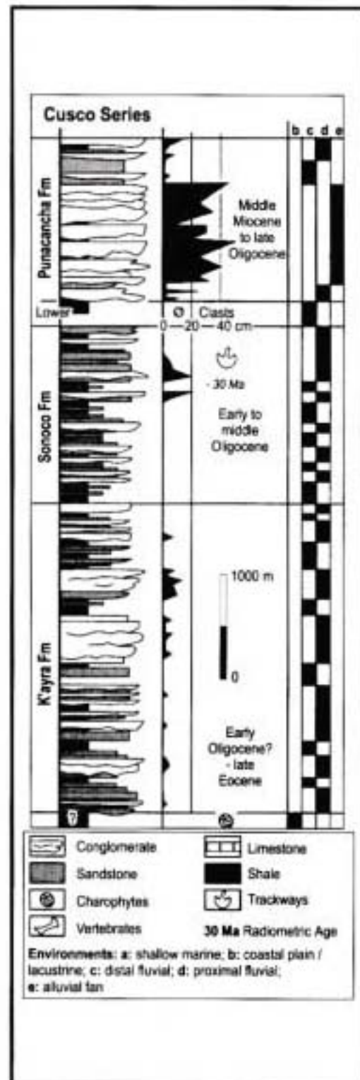
FIGURE 34 - Stratigraphic succession of the Eocene-Miocene "Red Beds" of the Cusco area (Andes of southern Peru) (after Carlotto, 1998).
