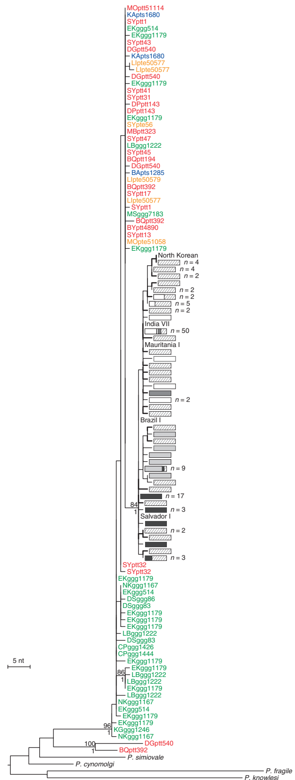
Figure 2 | Evolutionary relationships of ape and human P. vivax parasites in mitochondrial gene regions. The phylogenetic positions of mitochondrial fragment D (2,524 bp; Supplementary Fig. 1a) sequences from ape and human P. vivax strains are shown in relation to human and macaque parasite reference sequences. All sequences were generated by SGA 20 , except for human (Salvador I, India VII, Mauritania I, North Korean and Brazil I) and simian reference strains from the database (see Supplementary Tables 6–8 for GenBank accession numbers). Ape sequences are colour coded, with capital letters indicating the field site (Fig. 1) and lower case letters denoting species and subspecies origin (ptt: P. t. troglodytes , red; pte: P. t. ellioti , orange; pts: P. t. schweinfurthii , blue; ggg: G. g. gorilla , green). Human sequences are depicted by haplotype (rectangles) and labelled according to their geographic origin in Oceania (light grey), Africa (white), South and Central America (black), South and Southeast Asia (striped) and the Middle East (dark grey). Haplotypes that include more than one sequence are indicated, with the numbers of sequences listed to the right. A second lineage of related parasite sequences from chimpanzee samples DGptt540 and BQptt392 likely represents a new Plasmodium species. The tree was inferred using maximum likelihood methods 56 . Numbers above and below nodes indicate bootstrap values ( \geq 70\% ) and Bayesian posterior probabilities ( \geq 0.95 ), respectively (the scale bar represents five nucleotide substitutions).
