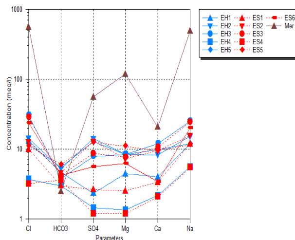
Figure 9: Schoeller diagram.
