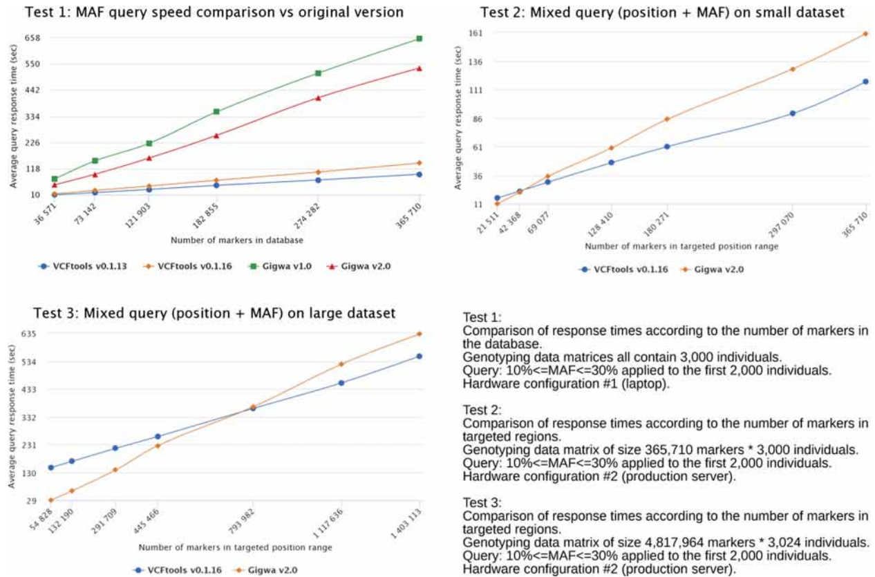
Figure 2: Benchmark results.
