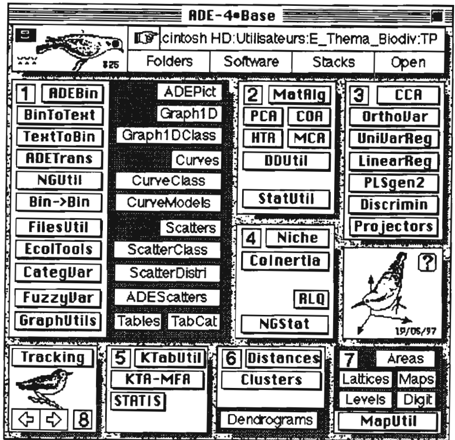
Figure 6: ADE-4 Hypercard (Macintosh) main interface. Computational modules appear in bold font and graphical ones in standard font. 1: File utilities, 2: One-table analyses, 3: Linear regression and two-table coupling methods, 4: Coinertia analysis, 5: k -table methods, 6: Distance and partitions, 7: Cartography modules.
