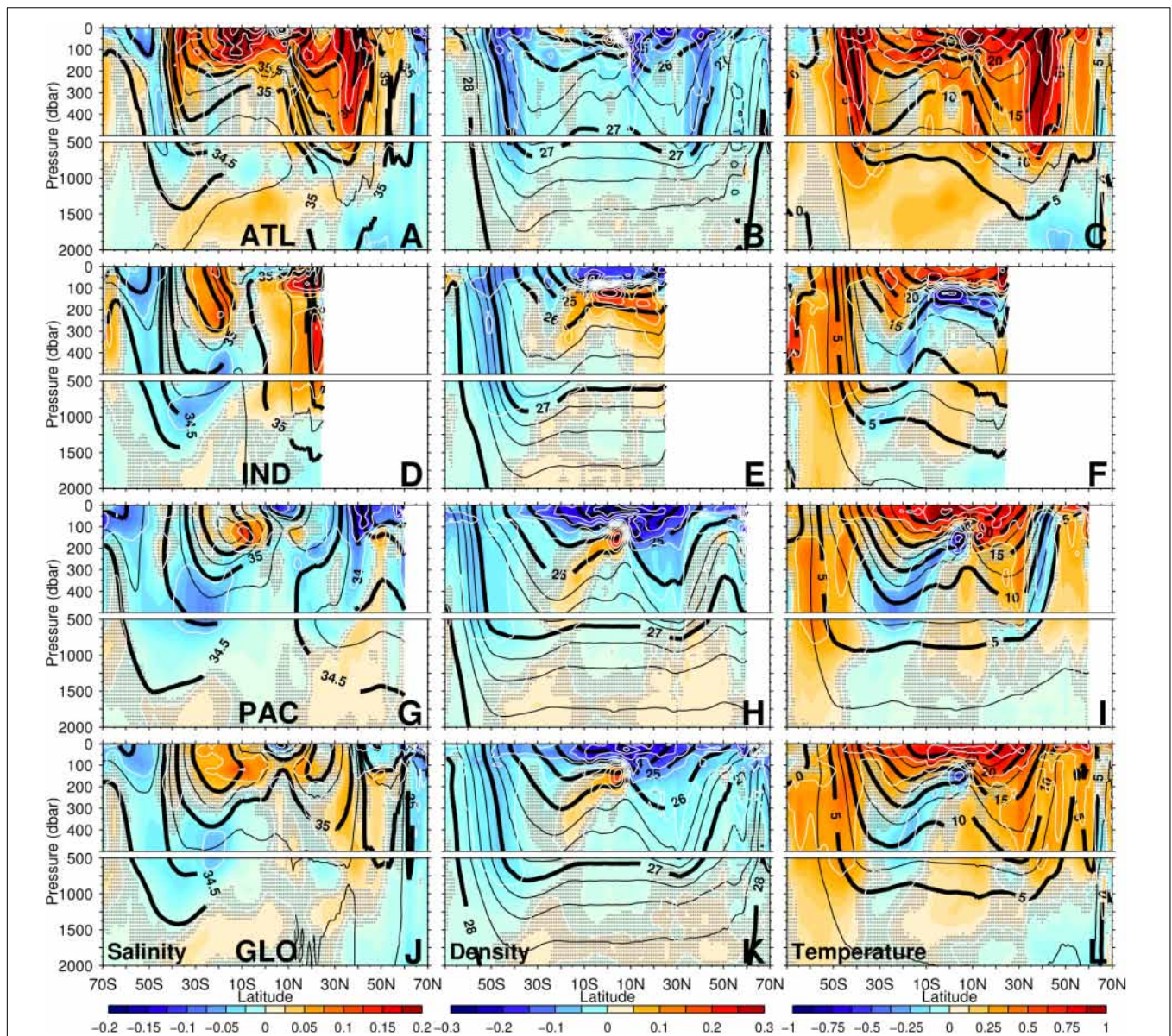
FIGURE 1 | Upper 2000 dbar (pressure) zonally averaged linear trend (1950–2000) (colors with white contours) of salinity changes (column 1, PSS-78 per 50 year; white contours: 0.05 PSS-78, –0.5 to 0.5), neutral density changes (column 2, \text{kg m}^{-3} per 50 year; white contours: 0.05 \text{kg m}^{-3} , –0.3 to 0.3), and potential temperature changes (column 3, ^{\circ}\text{C} per 50 year; white contours: 0.25 ^{\circ}\text{C} , –1 to 1), for the Atlantic Ocean (ATL) in row 1 (A–C), Indian Ocean (IND) in row 2 (D–F), Pacific Ocean (PAC) in row 3 (G–I), and global ocean (GLO) in row 4 (J–L). Mean fields are shown as black lines (Salinity: thick black contours 0.5 PSS-78, thin contours 0.25 PSS-78; Neutral density: thick black contours 1.0 \text{kg m}^{-3} , thin contours 0.25 \text{kg m}^{-3} ; Potential temperature: thick black contours 5.0 ^{\circ}\text{C} , thin contours 2.5 ^{\circ}\text{C} ). Trends are calculated on pressure surfaces. Regions where the resolved linear trend is not significant at the 90% confidence level are stippled in gray. Reproduced from IPCC AR5 (Rhein et al., 2013, Figure 3.9).
