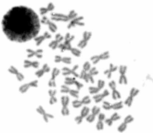
Fig. 4c : Gerbillus pyramidum (2n=38 NFa=72)
