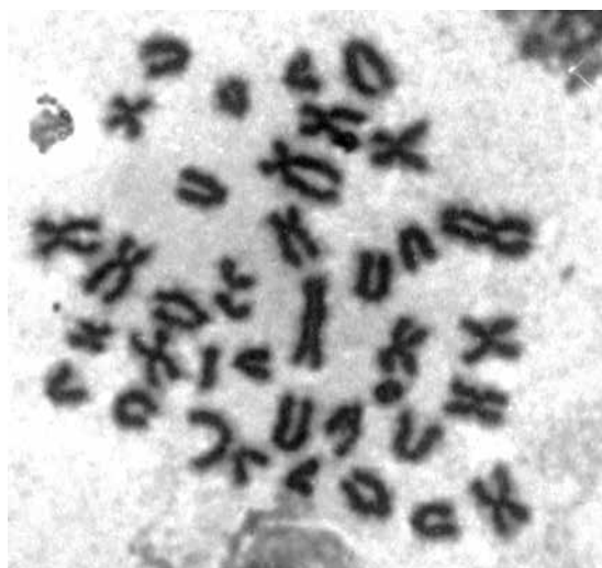
Fig. 2c : Mastomys erythroleucus (2n=38 NFa=50)
