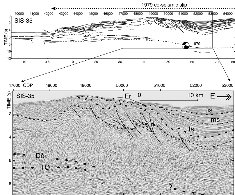
Figure 10. Multichannel seismic reflection line SIS-35 across the middle ridge and forearc basin. Location is shown in Figure 3. (top) Line drawing with cross-margin extent of 1979 coseismic slip. The 1979 focal mechanism [Kanamori and McNally, 1982] has been projected onto the line at a depth chosen to coincide with the plate interface according to seismic reflection data. (bottom) Close-up showing shortening distributed across the margin wedge and forearc basin. Er is a recent unconformity; ls, ms, us, Dé, and TO are as in Figure 6.
