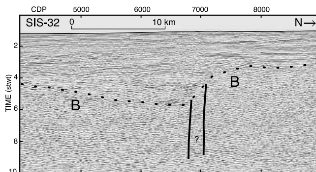
Figure 7. Multichannel seismic reflection strike line SIS-32 along the forearc basin. Location is shown in Figure 3. The line shows a thick sedimentary fill overlying a deformed basement B.
