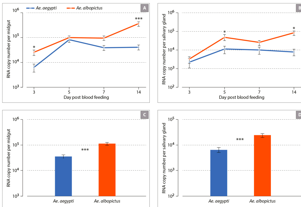
Figure 2. Kinetics of Mayaro (MAYV) infection of Ae. albopictus and Ae. aegypti mosquitoes. Panels (A,B) represent the number of the viral genome across time in the midgut and salivary glands, respectively. Panels (C,D) represent the mean number of viral genome for all time points. Error bars represent the standard error of the mean and asterisks indicate the significance level for statistical difference between mosquito species: * p < 0.05 ; *** p < 0.001 ; non-significant differences were not indicated for clarity.
