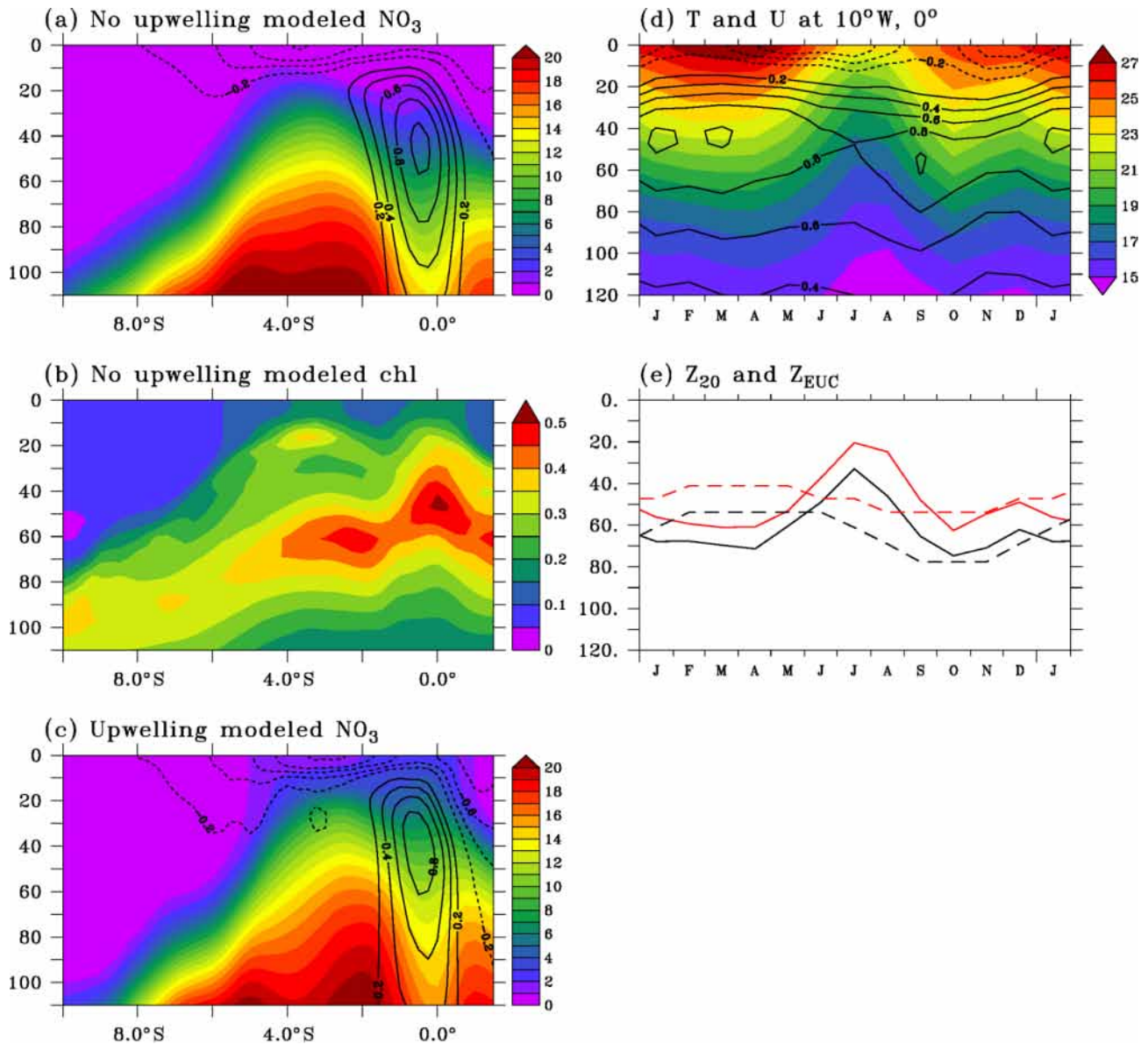
Figure 4. (a, c) Simulated nitrate ( \mu\text{mol L}^{-1} ) and chlorophyll ( \text{mg m}^{-3} ; b) distributions along 10°W during low-productivity (a, b) and high-productivity (c) conditions. Zonal velocity is overlaid on nitrate distribution. (d) Seasonal cycles of temperature (colors; °C) and zonal current (contours; \text{m s}^{-1} ) at 0°N, 10°W. Velocity contour interval is 0.2 \text{ m s}^{-1} ; the 0 \text{ m s}^{-1} contour has been removed. (e) Observed (black) and simulated (red) depths of the 20°C isotherm (full line) and of the EUC core (dashed line) at 0°N, 10°W.
