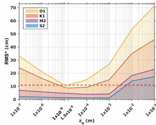
Figure 10. Model complex errors (Appendix; Eq. A2) relative to altimetry data for tests performed with varying the values of the uniform z_0 over the domain (SET2). The space in between two lines corresponds to the error for each wave. The yellow line corresponds to the cumulative errors for all four waves. The dashed red line corresponds to the smallest cumulative error, here equal to 10.96 cm and obtained for z_0 = 1.5 \times 10^{-5} m.
