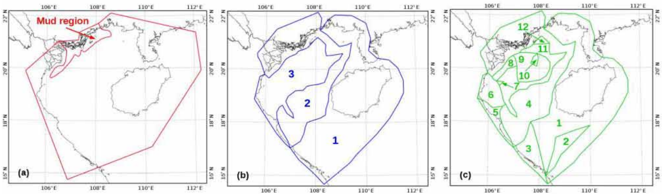
Figure 12. Spatial partitioning of the domain for the set of experiment SET3 (a), for SET4 (b), and for SET5 (c).
