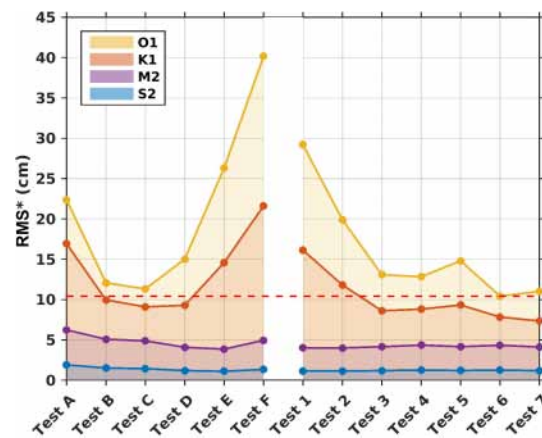
Figure 13. Model complex errors (Appendix; Eq. A2) relative to altimetry data for tests listed in Table 1 performed with nonuniform values of z_0 (SET3 and SET4). The space in between two lines corresponds to the errors for each wave. The yellow line corresponds to the cumulative errors for all four waves. The dashed red line corresponds to the smallest cumulative error, found for Test 6 (SET4), equal to 10.43 cm.
