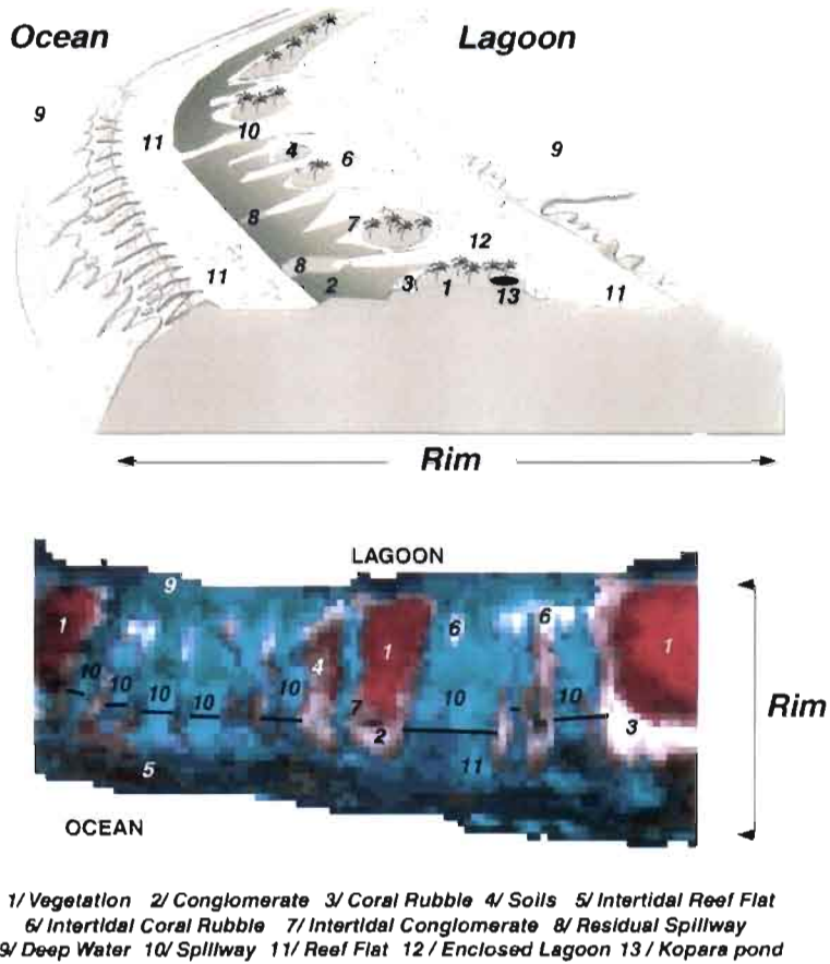
Figure 2. Bloc-diagram of an atoll rim (from Battistini et al. 1975) displaying the 13 classes at the Integrated level of description. The classes are also readily visible on a SPOT HRV image of the rim of the Tikehau atoll. The black segments indicate the locations of the apertures in this rim with numerous spillways. The aperture A is simply the sum of the width of these segments.
