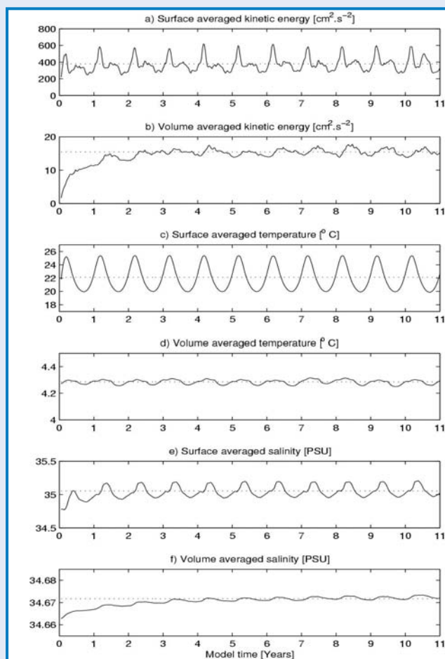
Figure 2. Time evolution of different model variables: a) Surface averaged kinetic energy ( \text{cm}^2.\text{s}^{-2} ), b) Volume averaged kinetic energy ( \text{cm}^2.\text{s}^{-2} ), c) Surface averaged temperature ( ^{\circ}\text{C} ), d) Volume averaged temperature ( ^{\circ}\text{C} ), e) Surface averaged salinity (PSU), and f) Volume averaged salinity (PSU)
