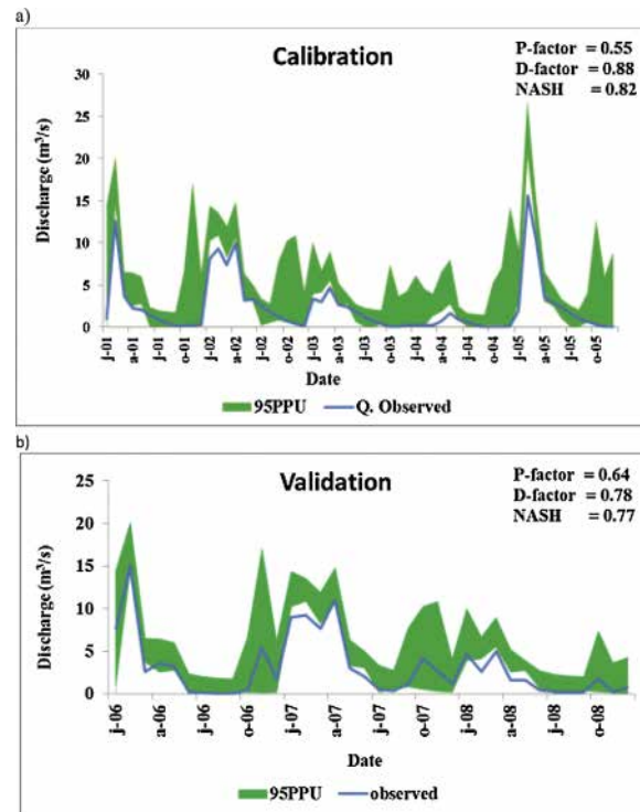
Fig. 4. Monthly runoff calibration/validation.
