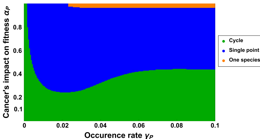
FIGURE C1 Phase transition diagram representing the community structure as a function of the cancer's impact on fitness \alpha_p and the occurrence rate of cancer \gamma_p . Cancer is present only in the predator population. The trade-off considered is between occurrence rate of cancer \gamma_p and energetic conversion e
