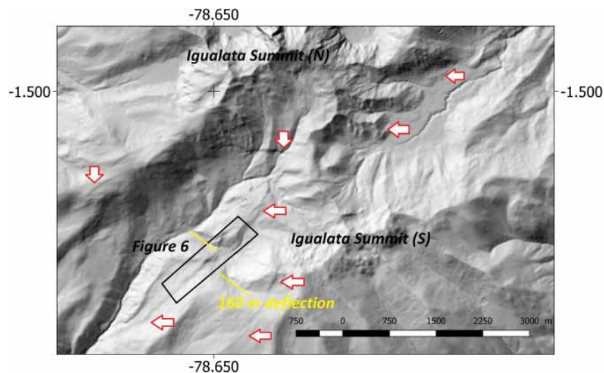
FIGURE 5 | Zoom-in of the Iguata center area. The figure highlights several sharp scarps and deflecting lineaments across the covered area, along the red arrows. The figure focuses on the lineament that includes the Figure 6 features and that seems to cause the 160 m right lateral deflection of the major incision (underlined in yellow).
