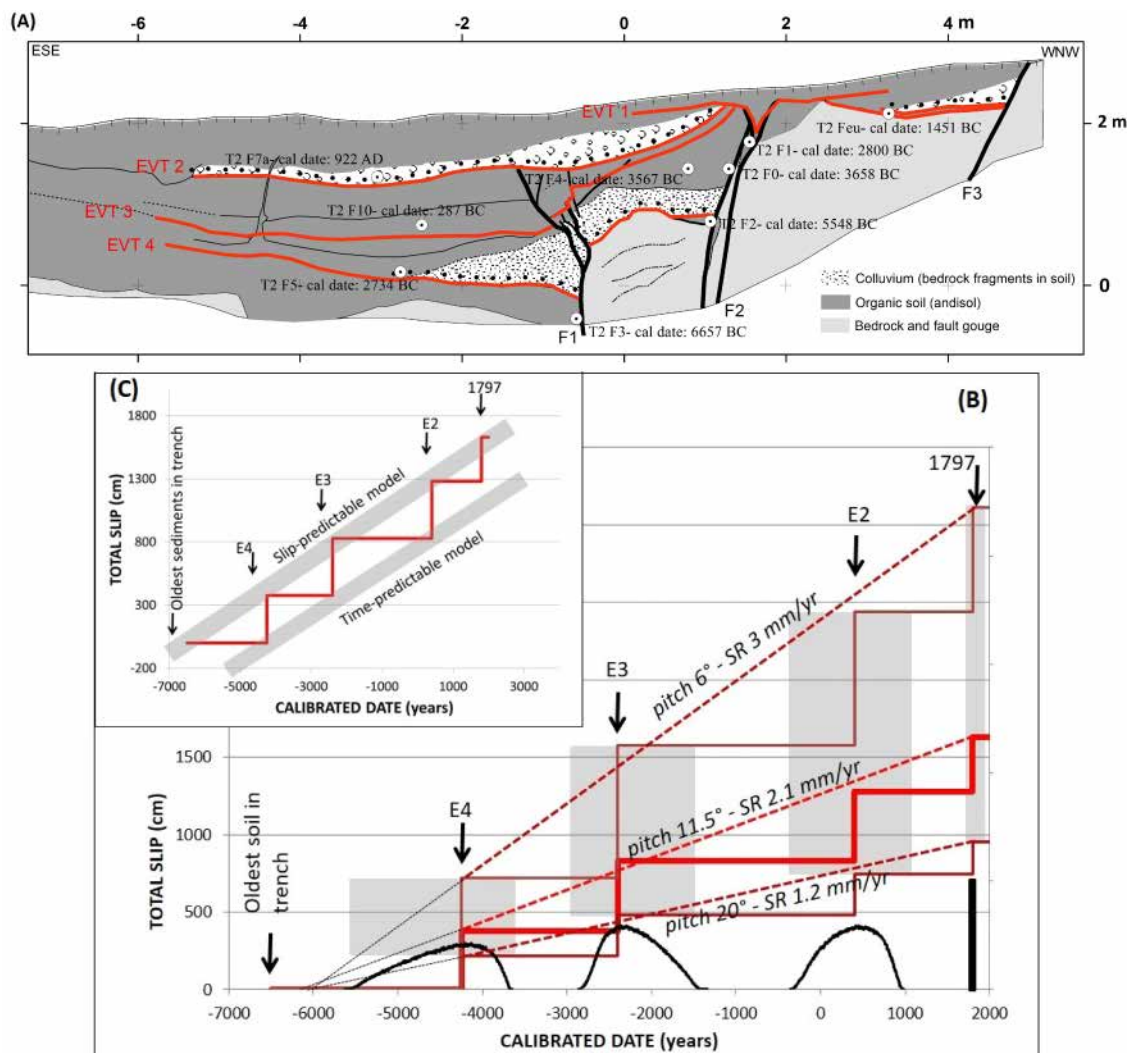
FIGURE 12 | Illustration of the slip versus time history inferred from the Rumipamba trench results. (A) Geological section of trench T2 dug in 2009 in Rumipamba (Baize et al., 2015). We simplified the drawing in representing in a same caption the bedrock fragment-rich horizons (colluvial wedges), the soil units and the bedrock, as well as the fault planes and surrounding shattered rocks. We underline the stratigraphic location of the event horizons that are used in the OxCal analysis.
