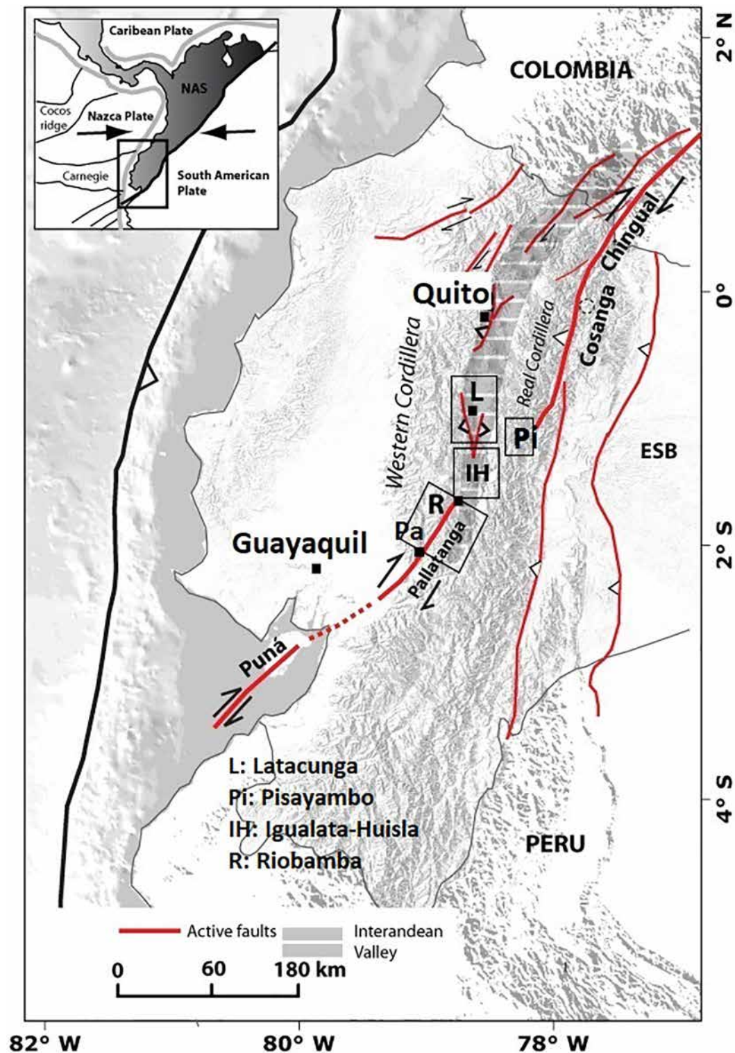
FIGURE 1 | Location of the investigated area in its tectonic context. Upper left inset gives a general geodynamic overview illustrating the major role of the CCPP (Chingual Cosanga Pallatanga Puna) fault zone acting as a boundary between the South America Plate and the North Andean Sliver (NAS) (Modified from Alvarado et al., 2016) in gray. The major active faults are the bold red lines; the investigated sectors are the Pallatanga fault north of Pallatanga (Pa) and south of Riobamba (R), the fault segments cutting the Igualata and Huisla volcanoes (IH) and the fault continuation around the Laguna Pisayambo (Pi) and the fault-related folds nearby Latacunga (L). (I) is Ibarra. The offshore bold line represents the subduction trench location, more than 100 km west of the Puna segment fault. ESB: Eastern Subandean Belt.
