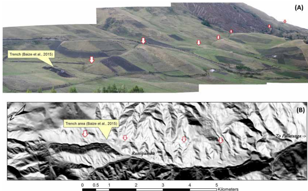
FIGURE 2 | Illustration of the signature of an active portion of the Pallatanga fault on a field panorama (A) and on the corresponding 4 m resolution DEM (B). On the left of the photo in (A), one can observe one of the trenches dug in 2009–2010 and presented in Baize et al. (2015). The fault trace is easily inferred from an uphill-facing and counter-slope scarp, matching a deflection in perpendicular morphological features (channel incisions, ridges). See Figure 3 and Supplementary Figure S8 for location.
