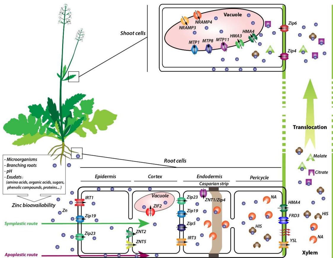
Figure 1. A model of the mechanisms that occur in hyperaccumulation plants upon exposure to zinc (Zn): Zn ion uptake, chelation, transport, and sequestration. Zn bioavailability can be influenced by several factors, such as microorganisms, branching roots, pH, and exudates. Once adsorbed by the roots, Zn can be absorbed by an apoplastic route: A passive diffusion through cells, or by a symplastic route via transporters. Within the latter path, Zn absorption by epidermis cells is mainly promoted by IRT1, ZIP19, and ZIP23. To reach the cortex, Zn can be directly diffused or by means of ZNT2 and ZNT5. Then, Zn can either be stocked in vacuoles (promoted by ZIF2) or transported to the endodermis through the following transporters: ZIP23, ZIP19, ZIP5, and IRT3. Zn following the apoplastic route is stopped by the casparian strip, and then enters the endodermis via ZNT1/ZIP4. At this level, Zn can be chelated by nicotianamine (NA) or directly diffused to pericycle cells where a part can also be associated to histidine (His). The unchelated Zn can reach the xylem through direct diffusion or via YSL, ferric reductase defective 3 (FRD3), and HMA4. Zn then crosses the xylem as a Zn-free form or coupled with His, citrate, or malate. To enter the leaf cells, Zn can passively penetrate in chelated forms or as the Zn-free form via ZIP4 and ZIP6 proteins. It is then sequestered inside the vacuole through MTP1 (metal tolerance proteins 1), MTP8, MTP11, NRAMP3, NRAMP4, HMA3, and HMA4 transporters, or blocked in the cell wall.
