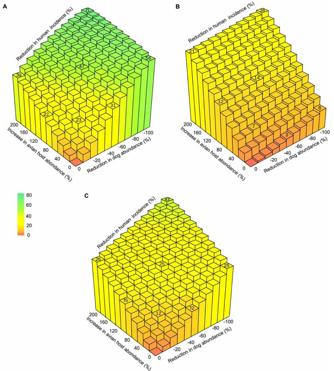
Fig 6. Zooprophyllaxis and its potential to limit T. cruzi transmission to humans in villages of the Yucatan peninsula. The maximal potential of zooprophyllactic interventions on human incidence is shown (A) along with their expected impact after 5 years (B) and 10 years (C). Interventions aim at reducing T. cruzi transmission by lowering the number of dogs (x-axis) or increasing the number of avian hosts (y-axis). The population sizes in the absence of intervention correspond to those observed in villages of the area and reported in Table 1.
