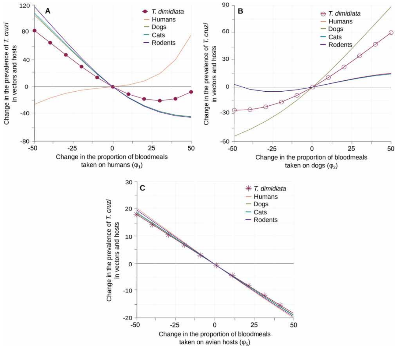
Fig 4. Impact of T. dimidiata blood-feeding preferences on the transmission of T. cruzi . Variation in the prevalence of T. cruzi infection in vectors and hosts are given with respect to changes in the proportion of blood meals taken on humans (A), dogs (B) and avian hosts (C). Changes in T. dimidiata prevalence of infection are indicated by circles (A-B) and crosses (C). Continuous lines describe variations in the different hosts prevalence of infection with the same host species colour code as in Fig 2.
