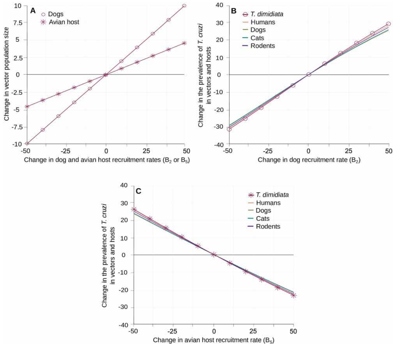
Fig 5. Impact of hosts demography and community structure on the transmission of T. cruzi . Variation in vector population size (A) and in the prevalence of T. cruzi infection in vectors and hosts (B-C) are given with respect to changes in the rate of recruitment (and abundance) in dogs ( B_2 ) and avian hosts ( B_5 ). Circles and crosses stand for the effects of B_2 and B_5 on T. dimidiata abundance (A) and its prevalence of infection by T. cruzi (B-C). Continuous lines describe variations in the different hosts prevalence of infection with the same host species colour code as in Fig 2.
