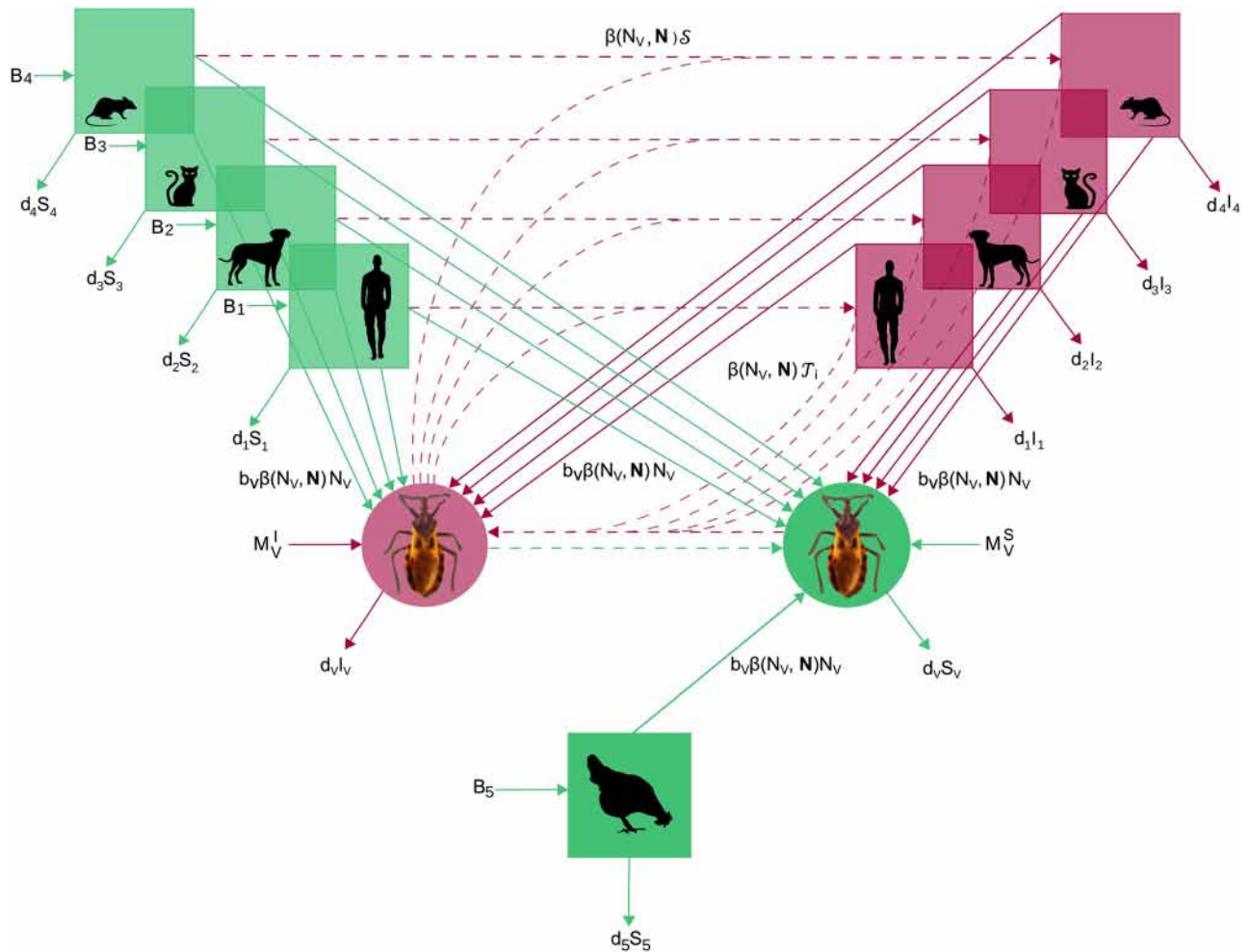
Fig 1. Flowchart for the SI model of T. cruzi transmission in a community of competent and non-competent hosts. Species i = 1 to 4 that are competent hosts (at the top) and vectors (in the middle) are made of susceptible (green) and infectious (red) individuals. Species 5 represents non-competent hosts (at the bottom) so that all individuals always remain susceptible (green). Arrows represent birth, death, migration and infection processes according to the parameters defined in the main text and Table 1. Continuous and dotted lines correspond to demographic and transmission processes. For simplicity, we used the notations S = \sum_{i \in C} \phi_i(N) \frac{d_i}{N_i} S_V p_V and T = \phi_i(N) \frac{d_i}{N_i} p_{IV} .
