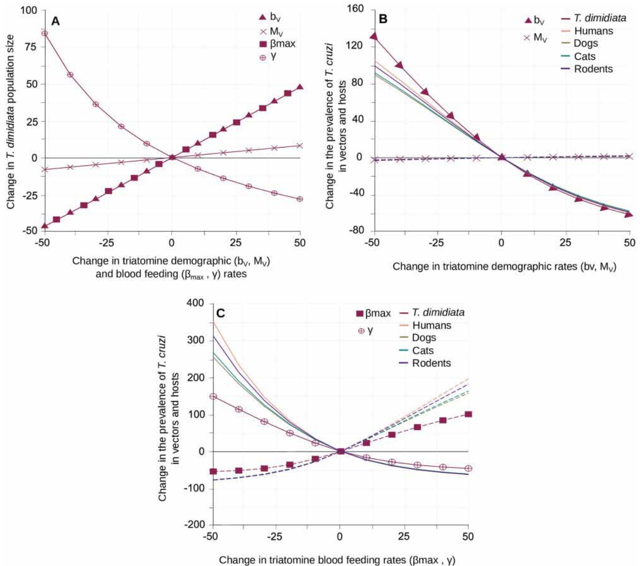
Fig 3. Impact of T. dimidiata demography and blood-feeding on the transmission of T. cruzi . Variation in vector population size (A) and in the prevalence of T. cruzi infection in vectors and hosts (B-C) are given with respect to changes in triatomine fertility ( b_v ), immigration ( M_v ), the level of competition for blood meals ( \gamma ) and in the maximal feeding rate ( \beta_{max} ). Triangles, crosses, circles and squared stand for the effects of b_v , M_v , \gamma and \beta_{max} on T. dimidiata abundance (A) and the prevalence of infection by T. cruzi in vectors (B-C). Continuous lines describe variations in the different hosts prevalence of infection by T. cruzi according to b_v (B) and \gamma (C), while (superimposed) dotted lines describe variation with respect to M_v (B) and \beta_{max} (C). Host species colour code is the same as in Fig 2.
