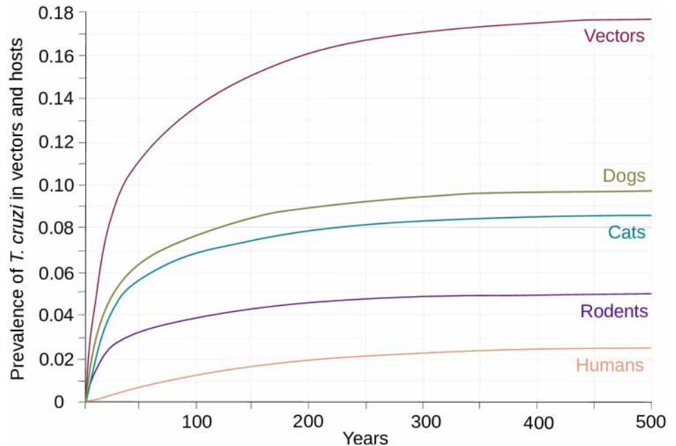
Fig 2. Dynamic of T. cruzi transmission in a village of the Yucatan peninsula. The dynamic of transmission was initiated by introducing parasite T. cruzi in its T. dimidiata vector. The prevalence of infection in the vector (purple) and in the competent hosts that include dogs (olive), cats (blue-green), rodents (indigo) and humans (salmon) were then followed until they reached asymptotic values corresponding to the endemic state of T. cruzi transmission typically observed in the villages of the Yucatan peninsula.
