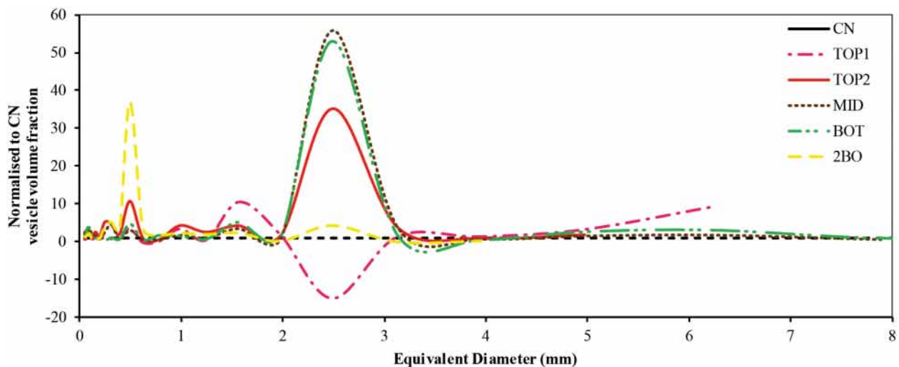
FIGURE 6 | Cumulative vesicle size distribution normalized to the control sample (CN). Most of the samples show an enrichment in vesicle size between 2 and 3 mm. TOP1 has seen a coalescence phenomenon which explains the depletion in the 2–3 mm range and increase > 5 mm (Thivet et al., 2020a).
