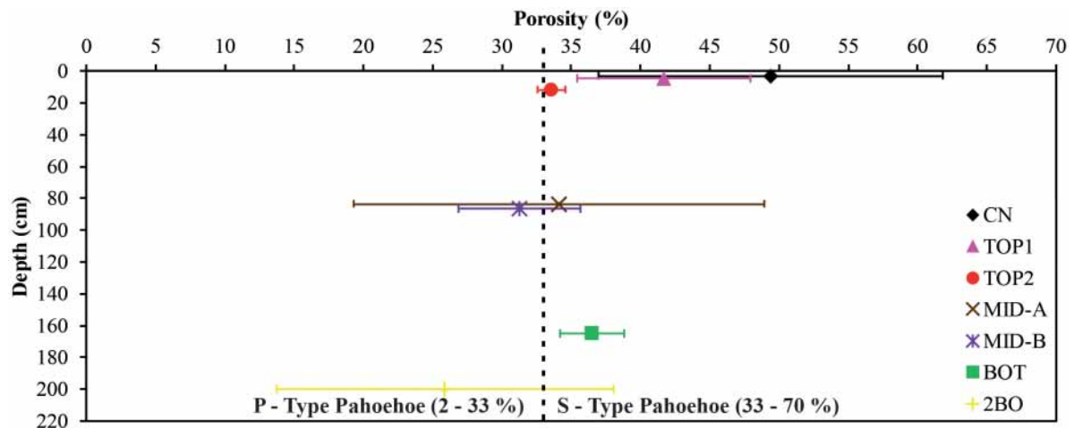
FIGURE 5 | Density-derived porosity as a function of depth in the mold (median value with range for each sample). The vertical-dashed line defines the porosity-defined limit between S-Type and P-Type pāhoehoe lava, as taken from data in Cashman et al. (1994), Harris and Rowland (2015), and Harris et al. (2017).
