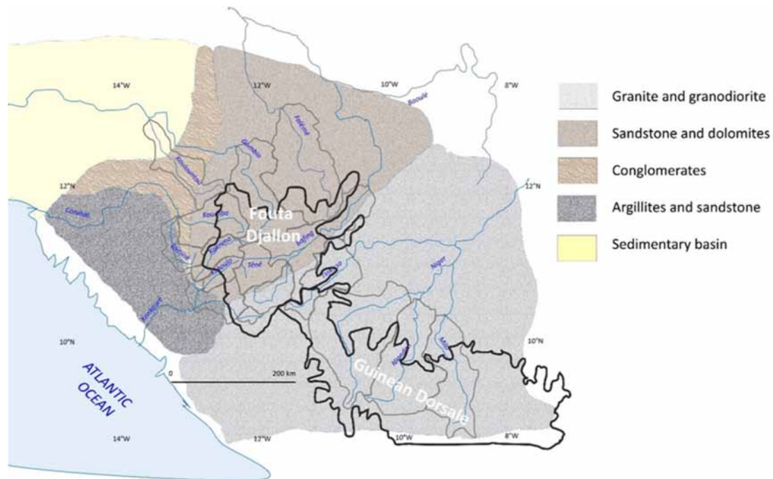
Figure 2. The main geological parts of the Fouta Djallon and Guinean Dorsale ensemble.
