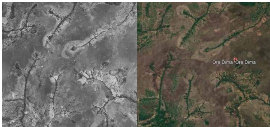
Figure 11. The so-called “three sources” area (15 km northward from Labé, the main city of the Fouta Djallon) in 1953 (IGN, left) and in 2019 (Google Earth©, right). No apparent deforestation. The extension of the picture is 5 km from the west to the east by 4.5 km from the north to the south. The area represented is the one of the red square in Figure 7.
