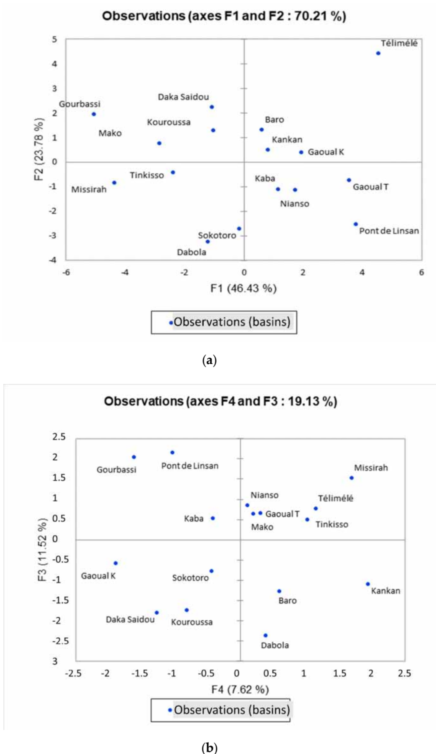
Figure 13. Observations spaces of the PCA analysis; (a): components 1 and 2; (b) components 3 and 4.
