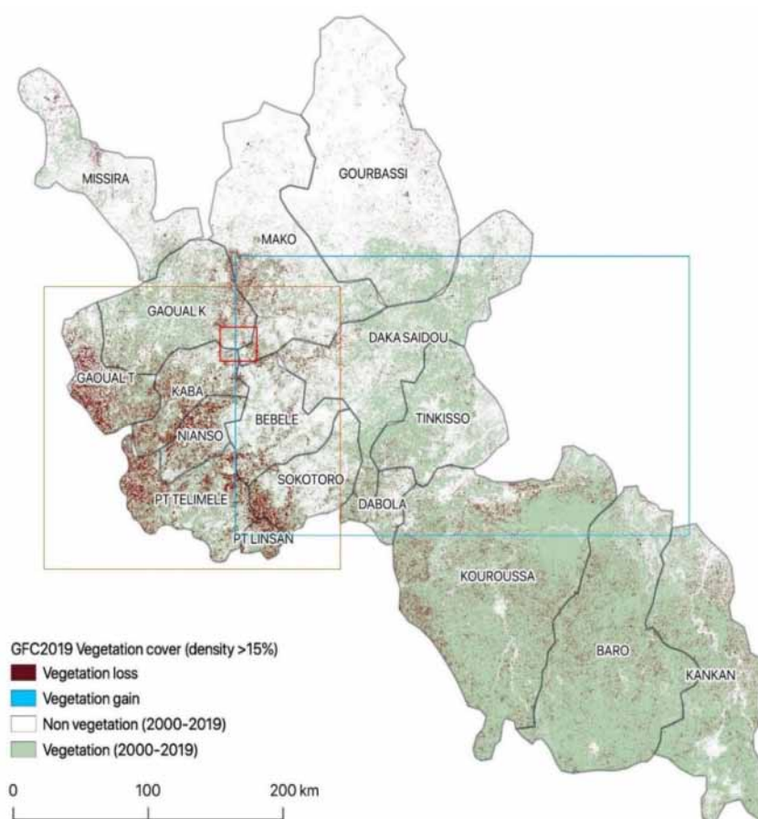
Figure 7. Vegetation (forest density higher than 15%) in 2000 and 2019 and vegetation loss and gain (GFC (Global Forest Change) product [29]), for the 16 basins. The empty brown rectangle is the area covered by the map in Figure 8.
