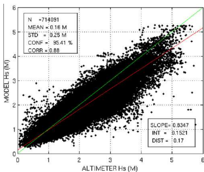
Fig. 3. Scatter-plot of collocated significant wave height ( H_s ) from altimetry and from the WAVEWATCH III model. Data were \pm 1 h 30 apart, corresponding to a spatial difference of 5–7 km at most. Data number (N), mean value (MEAN) and standard deviation (STD) of differences altimeter minus model H_s . Confidence level (CONF) and correlation (CORR). Slope and intercept (INT) of the inertial regression line, average distance to the line (DIST). Red: inertial regression line. Green: y = x line (For interpretation of the references to colour in this figure legend, the reader is referred to the web version of this article.).
