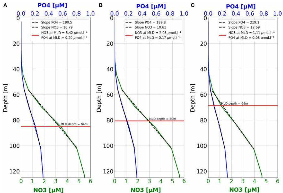
FIGURE 6 | Average profiles in autumn (September to November) of NO_3 (green) and PO_4 (blue) for the Western Basin for the periods: (A) 1986–2005; (B) 2021–2050; (C) 2071–2100. The red line shows the average mixed layers depth (MLD) in winter (January to March) for the same periods. Dotted lines show the linear relationship between nutrient concentrations and depth (green NO_3 and blue PO_4 ) between 60 and 100 m. These depths have been arbitrarily chosen in order to best represent the gradient regions of the nutriclines.
