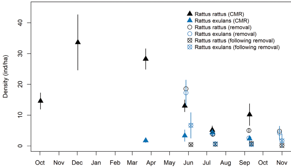
Figure 2. Density of rats ( \pm SE) in the study area from October 2014 to November 2015. Densities were estimated from the best SECR model ( g_0 \sim \text{indgr} + \text{session} , \sigma \sim \text{indgr} ) in the CMR area and from the Zippin removal method in the removal area.
