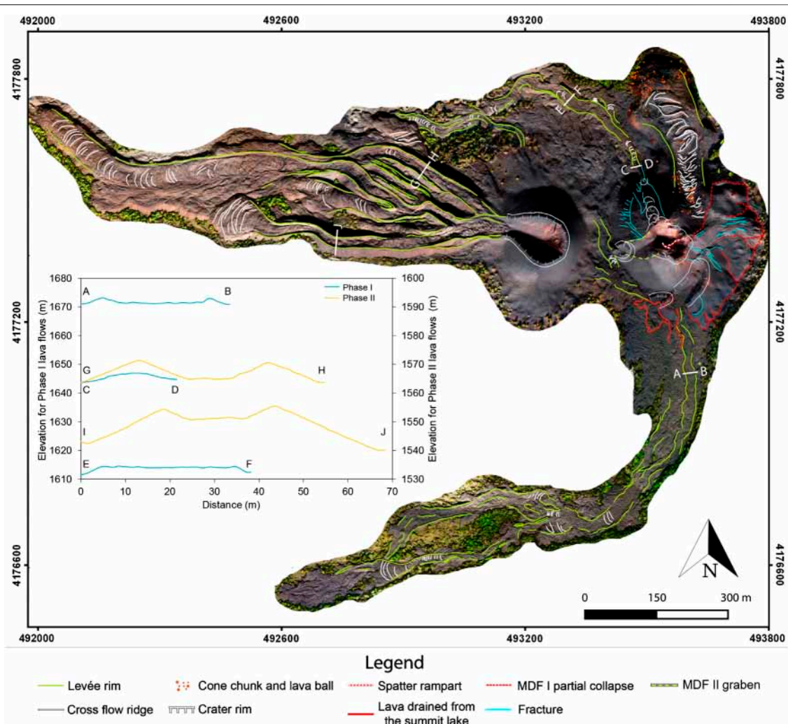
FIGURE 3 | Structural map of the January–March 1974 west flank eruption of Mount Etna overlain on the orthophoto of Favalli et al. (2018). Inset represents cross-unit profiles, taken perpendicular to flow direction, to show the overall shape of lava units associated with each phase: Profiles A–B (Unit 1.7), C–D (Unit 1.10, at vent) and E–F (Unit 1.10, medial) are for Phase I, and G–H (Unit 2.2) and I–J (Unit 2.4) are for Phase II.
