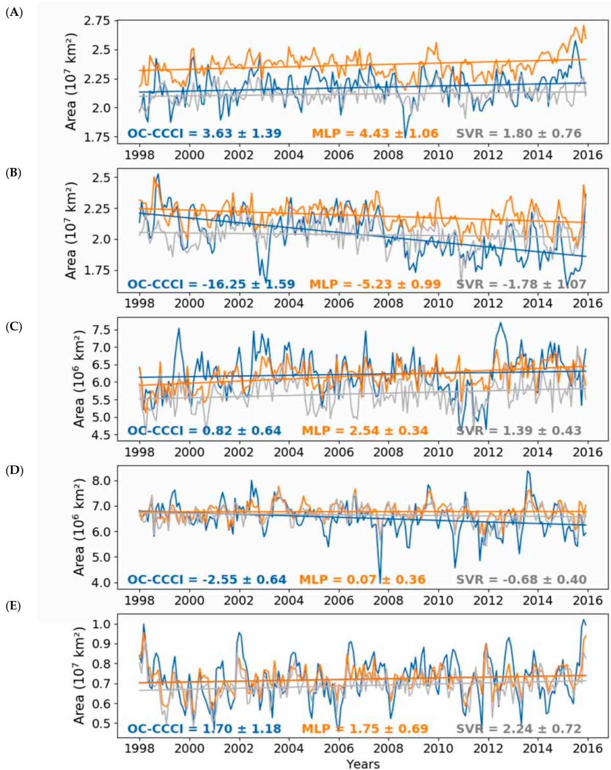
Figure 6. Time series of the monthly mean area ( \text{km}^2 ) with surface Chl less than or equal to 0.07 \text{ mg.m}^{-3} between 5^\circ and 45^\circ N/ ^\circ S latitude with the seasonal cycle removed in the (A) North Pacific, (B) South Pacific, (C) North Atlantic, (D) South Atlantic and (E) Indian Oceans. \text{Chl}_{\text{OC-CCI}} is in blue, \text{Chl}_{\text{SVR}} in grey and \text{Chl}_{\text{MLP}} in orange. Straight lines are the linear trends calculated as in Figure 5. The average trends and standard deviation are also indicated.
