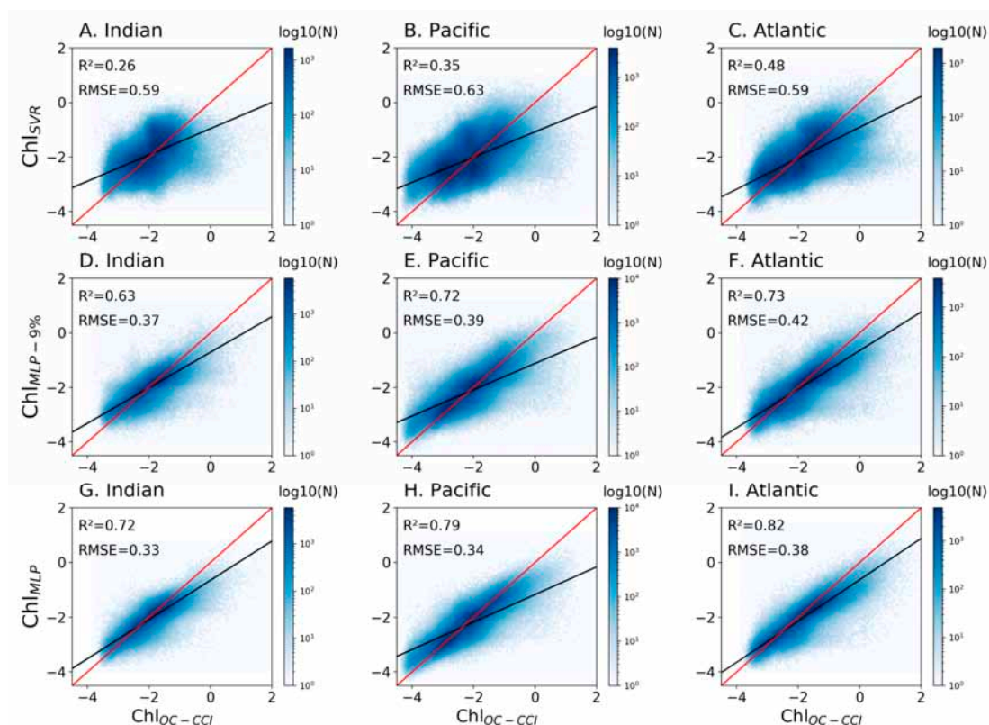
Figure 2. Scatter plots of log of Chl_{OC-CCI} vs. (A–C) Chl_{SVR} , (D–F) Chl_{MLP-9\%} and (G–I) Chl_{MLP} trained on 80% of the dataset, for each oceanic basin between 50^\circ S and 50^\circ N and over 1998–2015. The Chl_{OC-CCI} vs. reconstructed Chl regression lines are plotted in black and the 1:1 regression lines are plotted in red. The figure is color-coded according to the density of observations.
