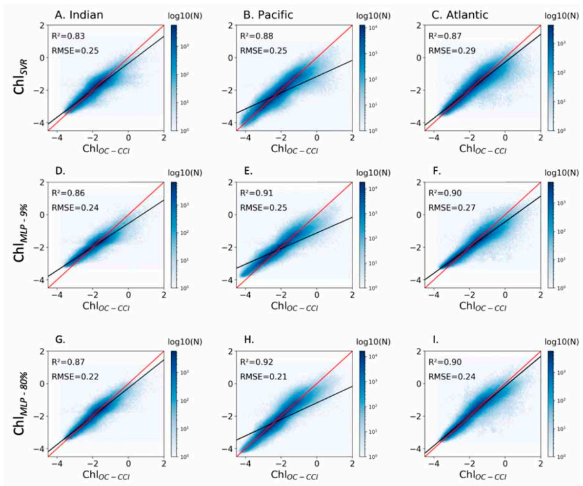
Figure 2. Scatter plots of log of Chl OC-CCI vs. (A–C) Chl SVR , (D–F) Chl MLP-9% and (G–I) Chl MLP trained on 80% of the dataset, for each oceanic basin between 50° S and 50° N and over 1998–2015. The Chl OC-CCI vs. reconstructed Chl regression lines are plotted in black and the 1:1 regression lines are plotted in red. The figure is color-coded according to the density of observations.
