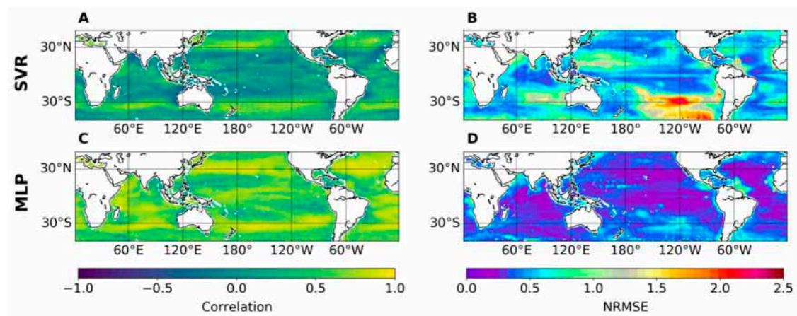
Figure 3. (A,C) Correlation and (B,D) NRMSE of \text{Chl}_{\text{OC-CCI}} vs. (up) \text{Chl}_{\text{SVR}} and (bottom) \text{Chl}_{\text{MLP}} over 1998–2015.
